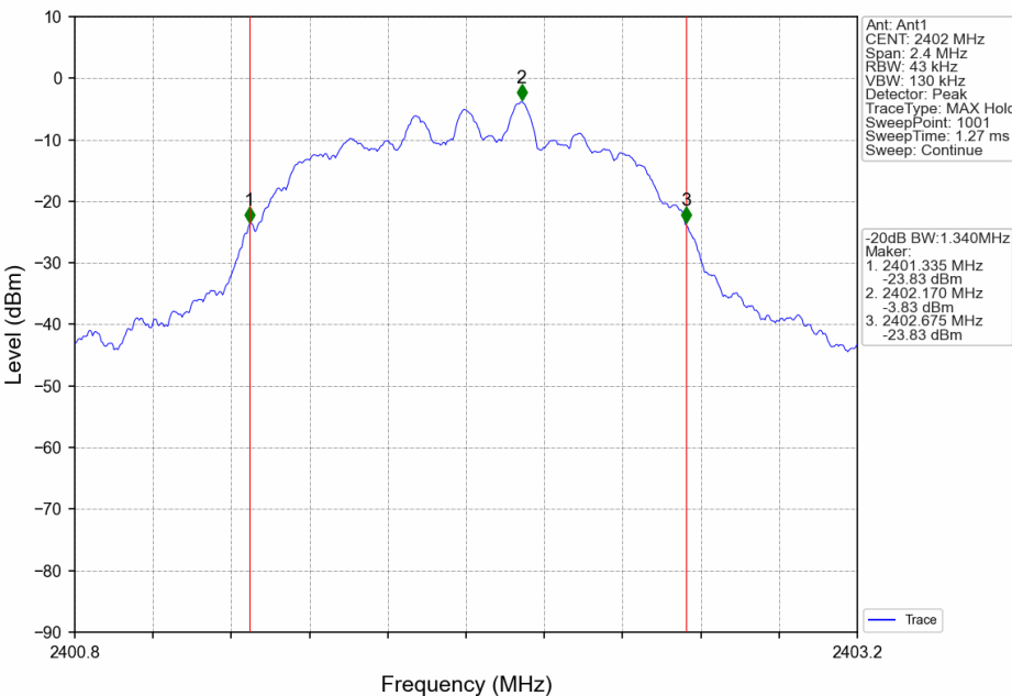
Pi/4DQPSK_2DH5_LCH_2402MHz_Ant1_NTNV
