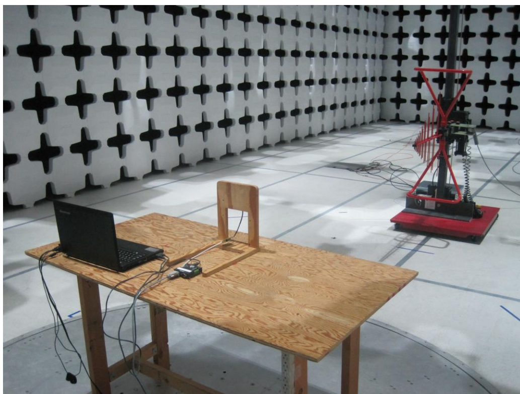
Radiated Emission Test setup (<1GHz) - Rear
