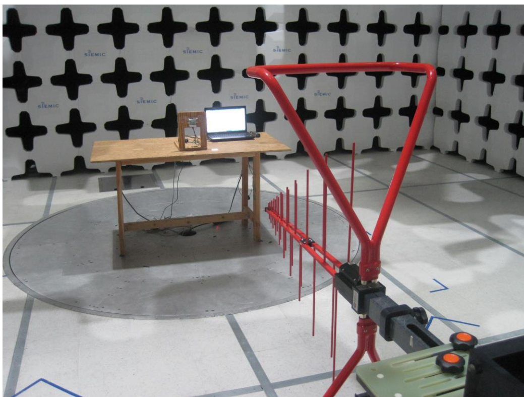
Radiated Emission Test setup (<1GHz) - Front
