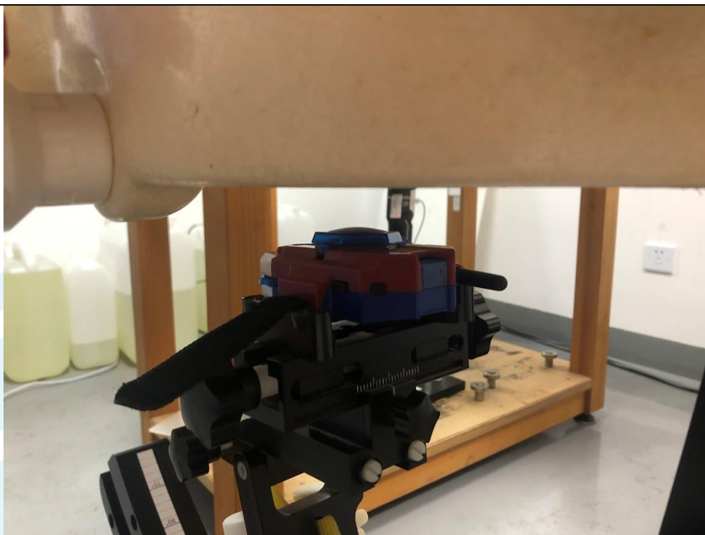
Front Face of EUT with 2.5 cm Gap
