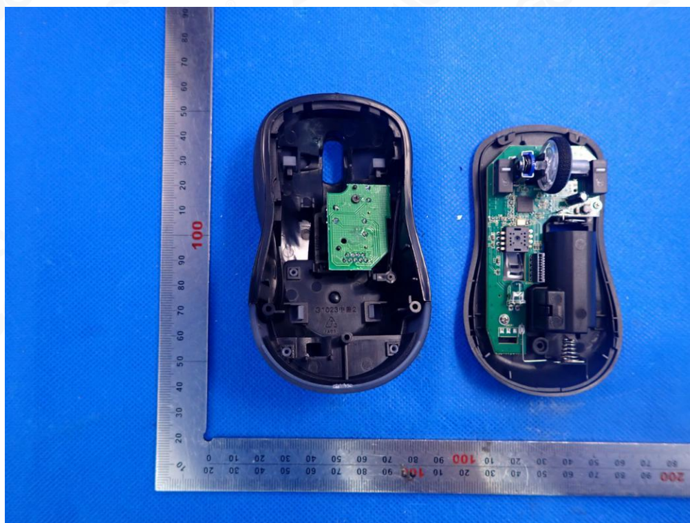
INTERNAL VIEW-1 OF EUT(D1023E)
