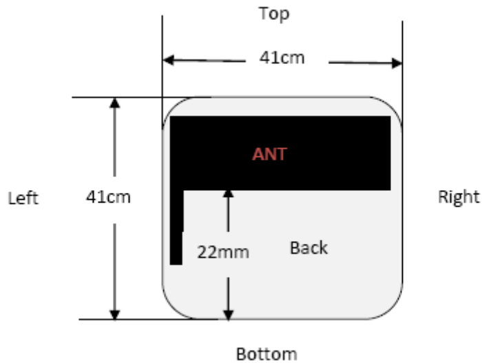
Fig.14.1 EUT Antenna Locations
