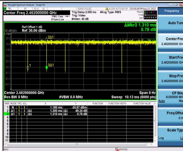
Keysight Spectrum Analyzer - Swept SA Center Freq 2.462000000 GHz Trig Delay: 2000 ms #Avg Time: RMS Frequency
