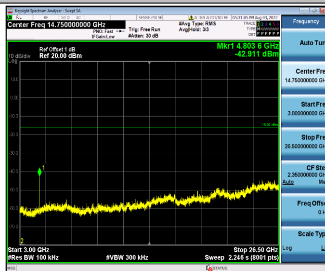
BLE_BT4.0_Ant2_2402_3000~26500
