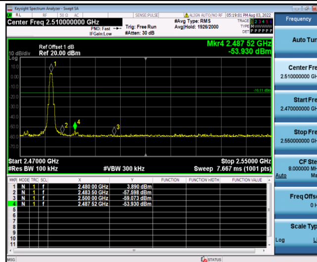
BLE_BT4.0_Ant1_High_2480
