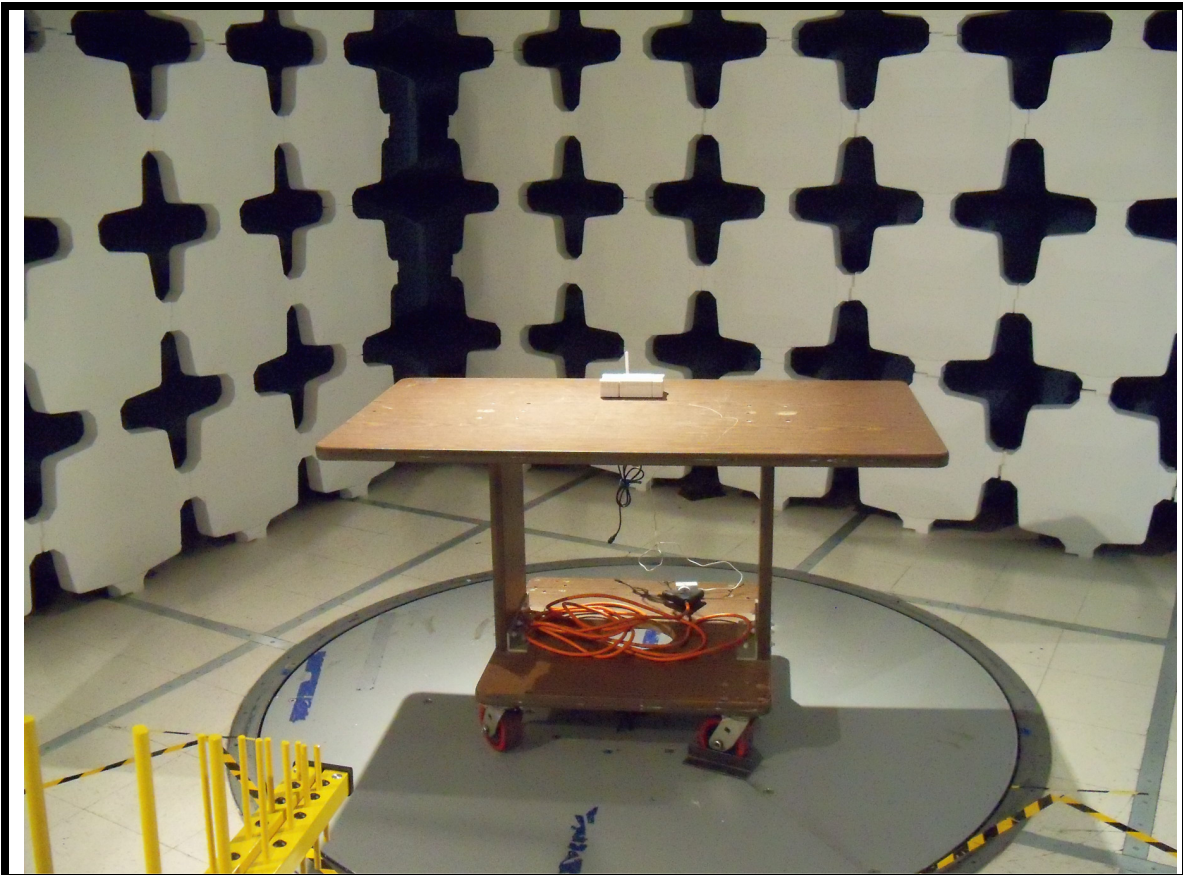
Photo 1 – Radiated Emissions
