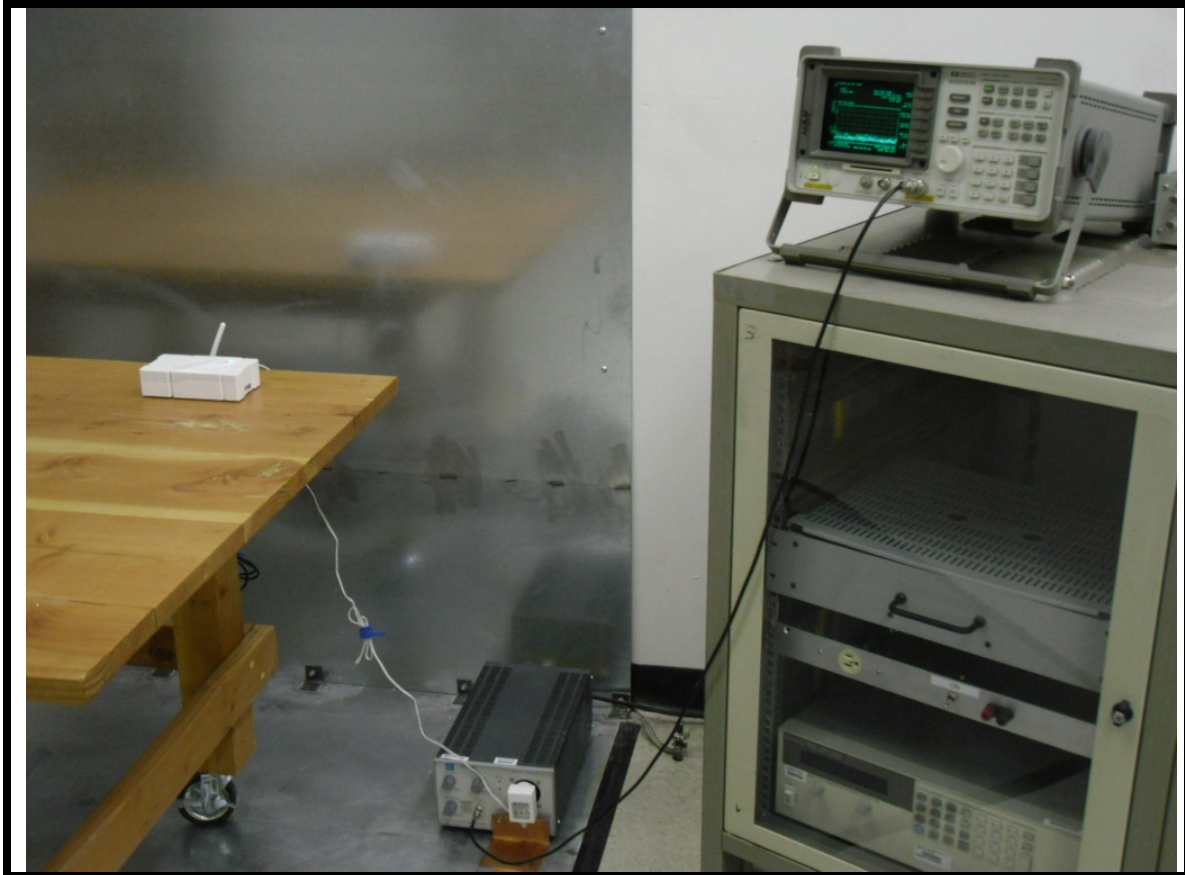
Photo 4 – Conducted Emissions
