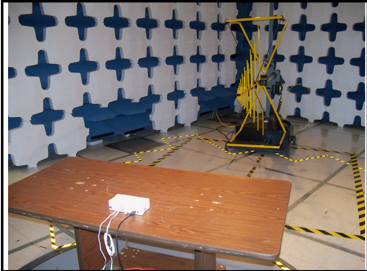
Photo 2 – Radiated Emissions
