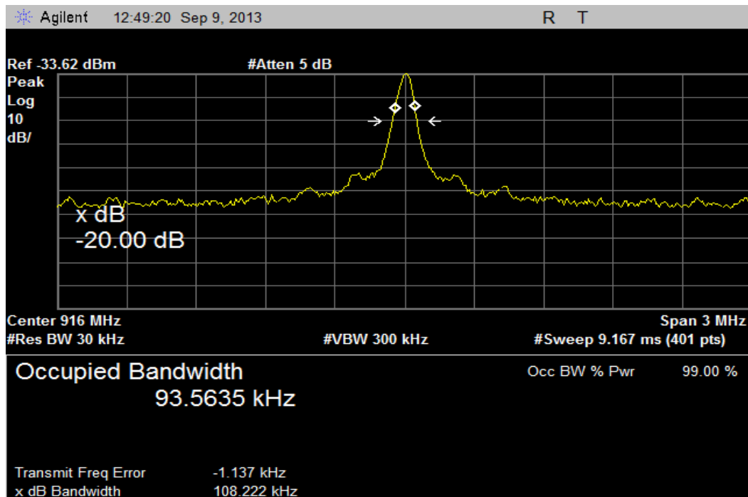
Plot 3 – 20dB BW FSK Modulation & 99% Occupied BW (For IC Only)
