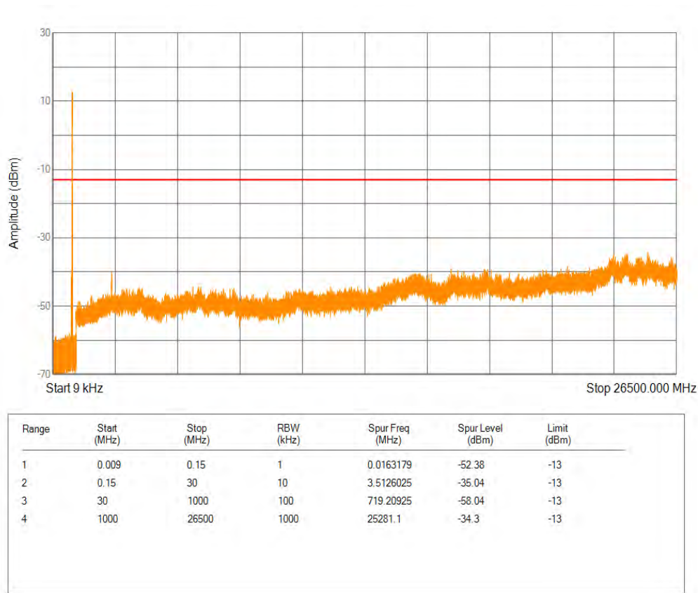
Band5 QPSK BW=10MHz Channel=20525 RB Size=50 Position=#0
