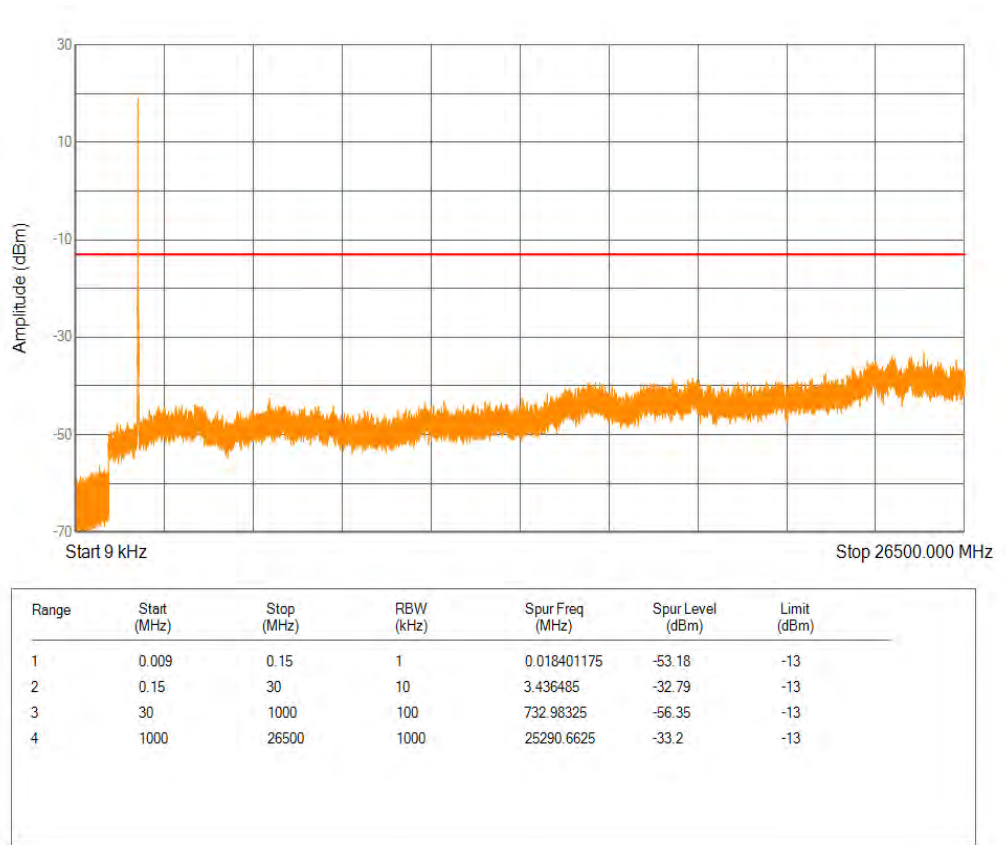
Band25 QPSK BW=10MHz Channel=26365 RB Size=50 Position=#0
