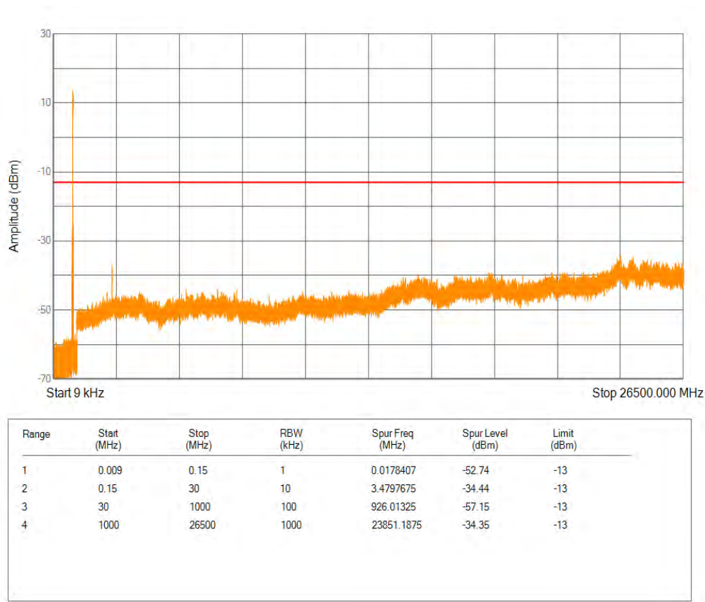
Band26(824-849) 16QAM BW=5MHz Channel=26815 RB Size=25 Position=#0
