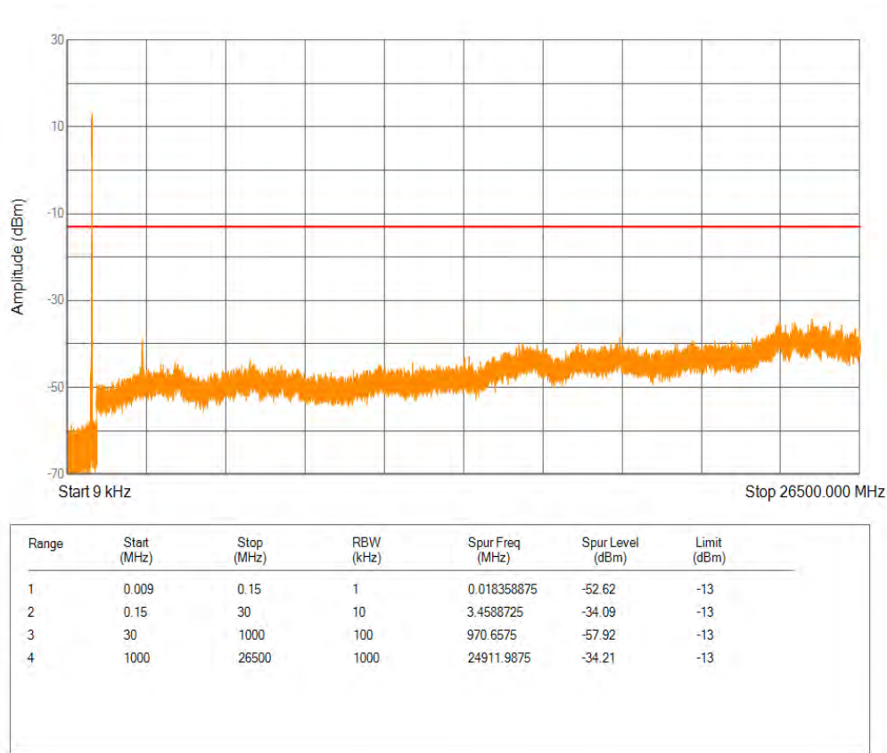
Band5 QPSK BW=10MHz Channel=20600 RB Size=50 Position=#0
