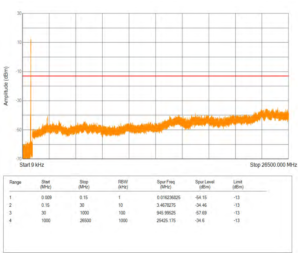
Band26(824-849) QPSK BW=10MHz Channel=26915 RB Size=50 Position=#0
