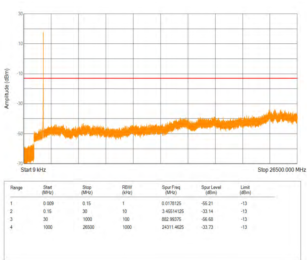
Band25 QPSK BW=15MHz Channel=26615 RB Size=75 Position=#0
