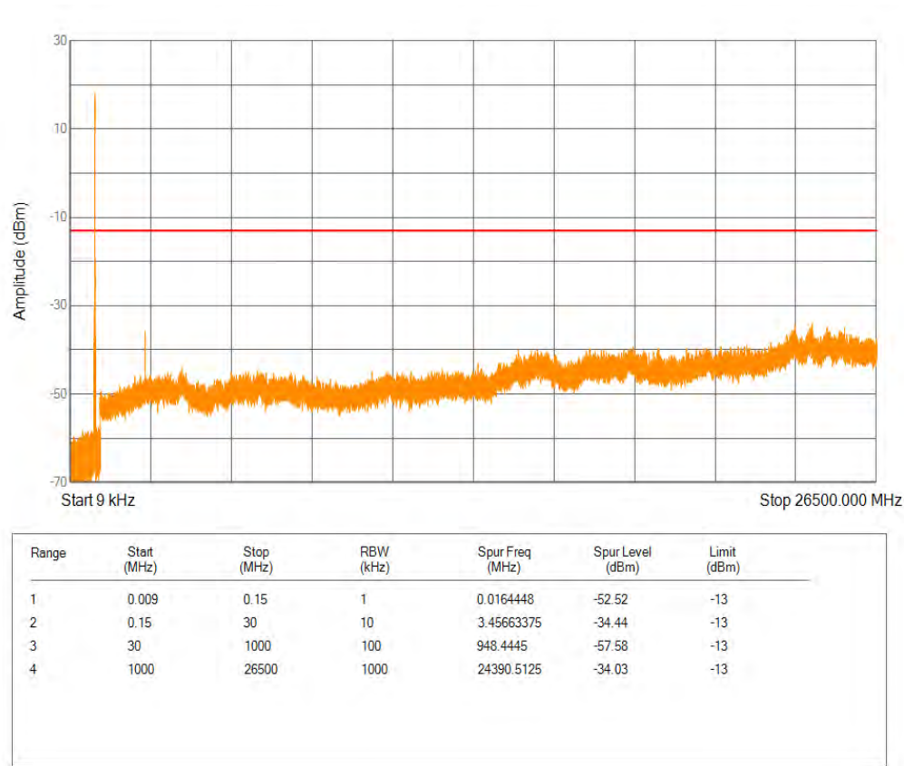
Band5 QPSK BW=3MHz Channel=20415 RB Size=15 Position=#0
