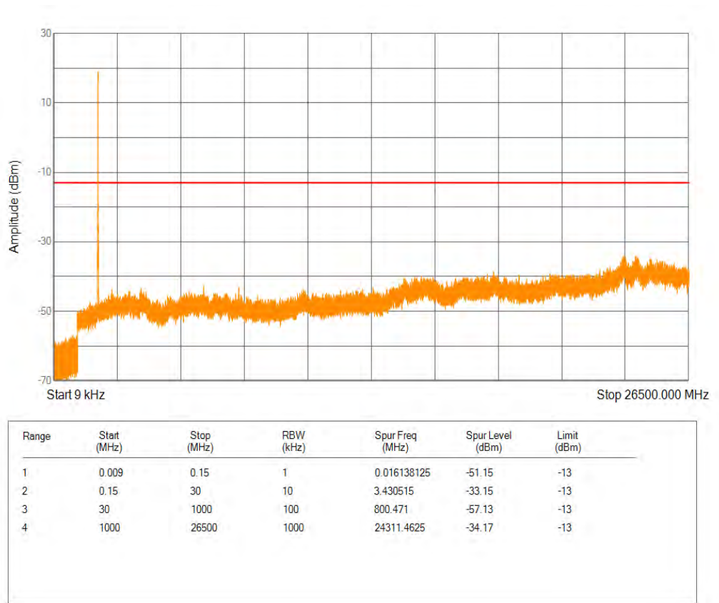
Band25 QPSK BW=10MHz Channel=26090 RB Size=50 Position=#0
