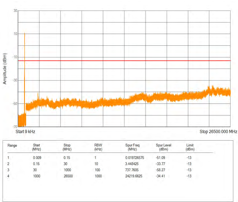
Band26(824-849) QPSK BW=15MHz Channel=26865 RB Size=75 Position=#0
