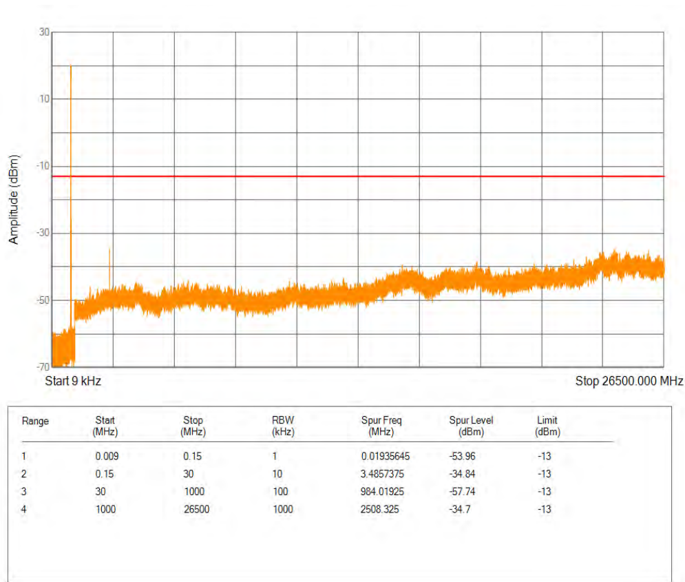
Band5 QPSK BW=1.4MHz Channel=20525 RB Size=6 Position=#0
