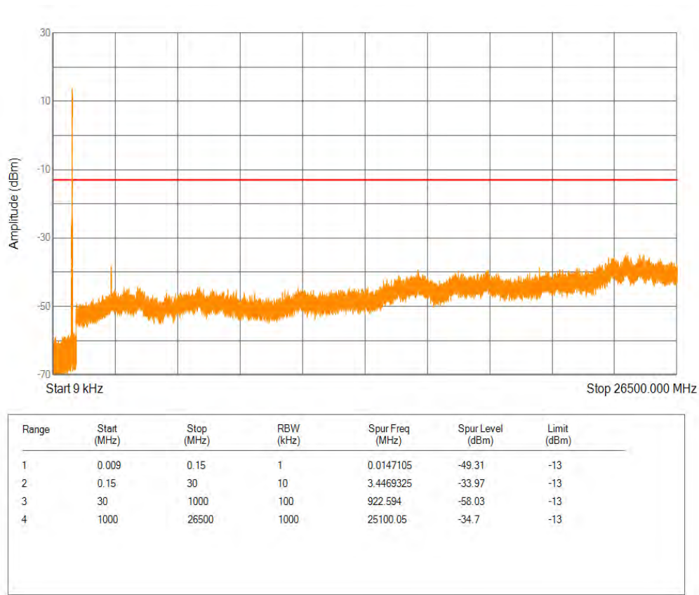
Band26(824-849) QPSK BW=10MHz Channel=26840 RB Size=50 Position=#0
