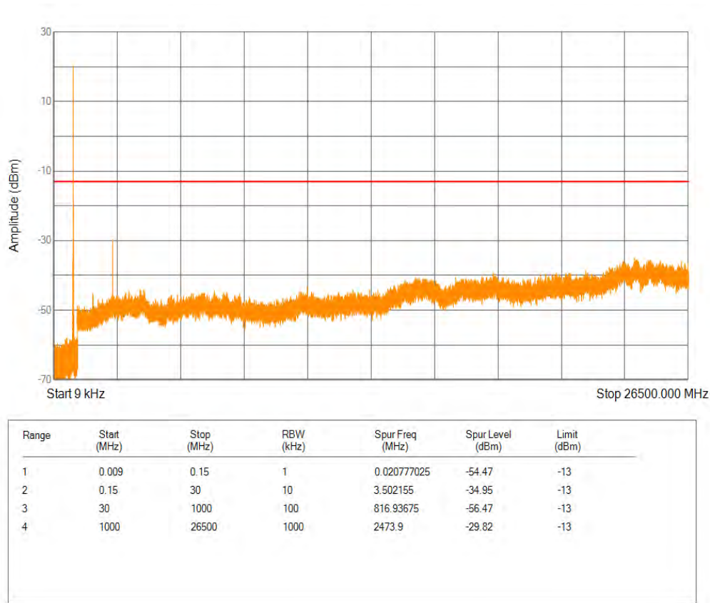
Band5 QPSK BW=1.4MHz Channel=20407 RB Size=6 Position=#0
