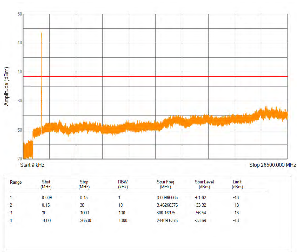
Band25 QPSK BW=15MHz Channel=26365 RB Size=75 Position=#0
