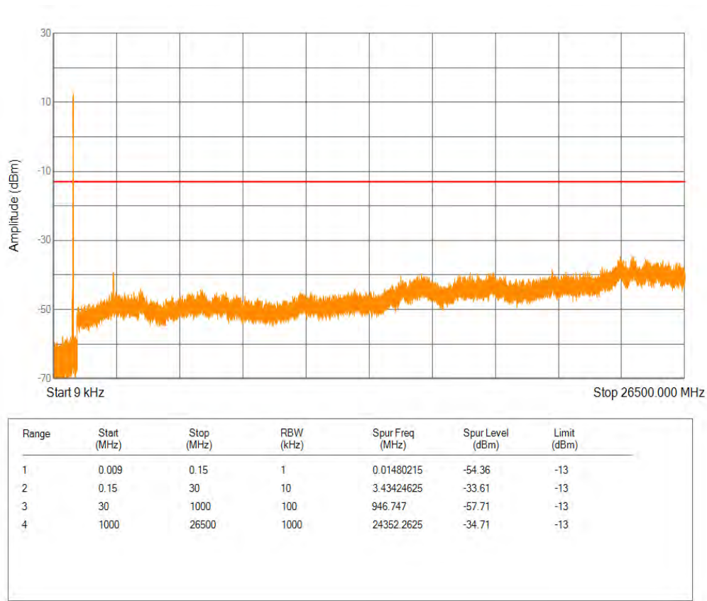
Band26(824-849) QPSK BW=10MHz Channel=26990 RB Size=50 Position=#0
