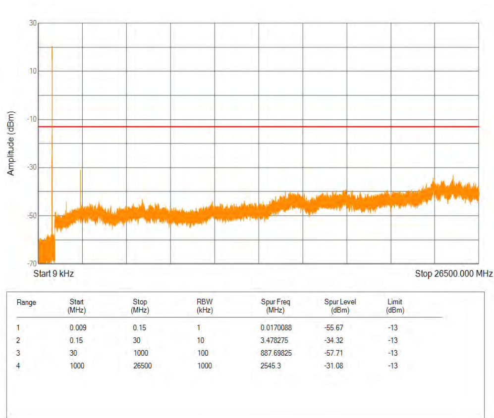
Band5 QPSK BW=1.4MHz Channel=20643 RB Size=6 Position=#0
