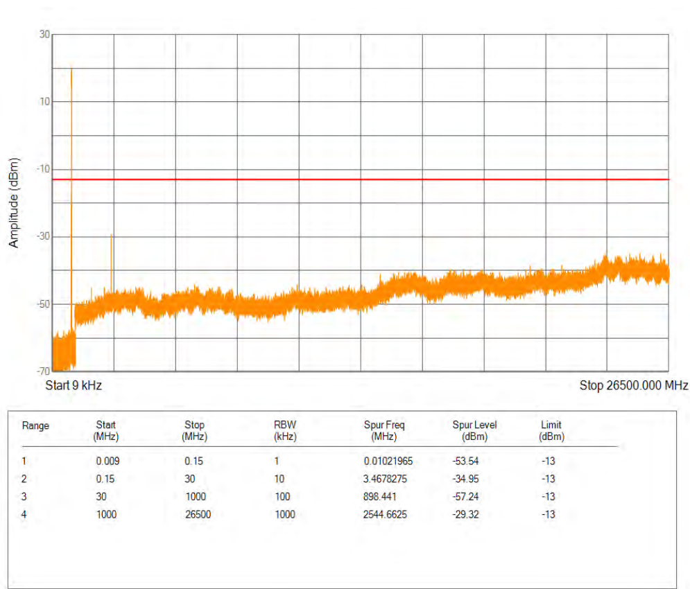
Band26(824-849) 16QAM BW=1.4MHz Channel=27033 RB Size=6 Position=#0
