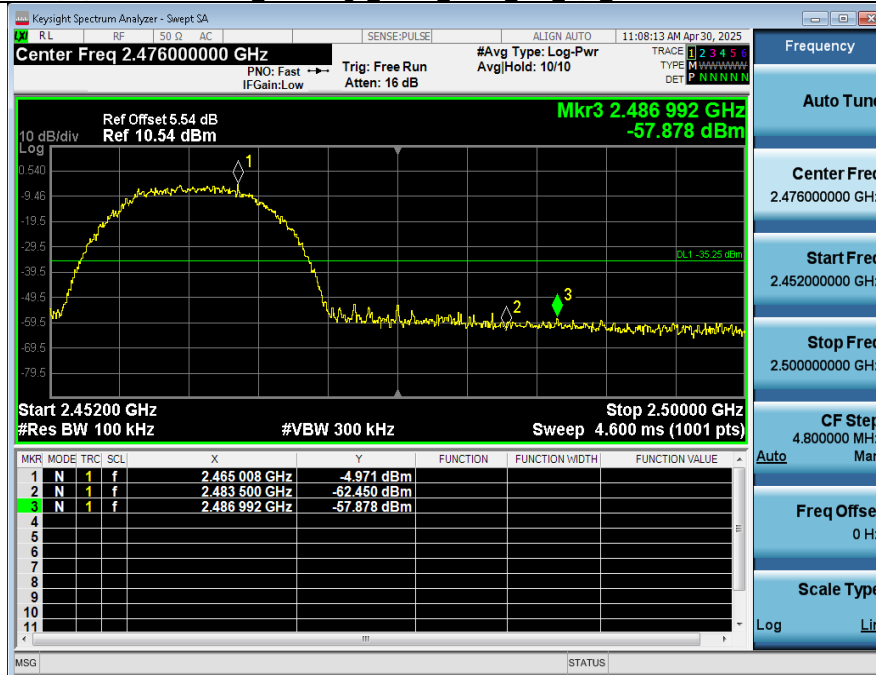
2_Bandedge_NVNT_ANT1_802_11b_2462
