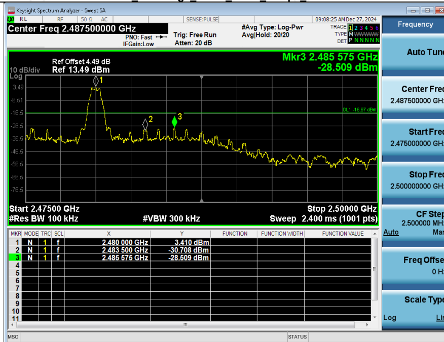
2_Bandedge_NVNT_ANT1_1Mbps_2480
