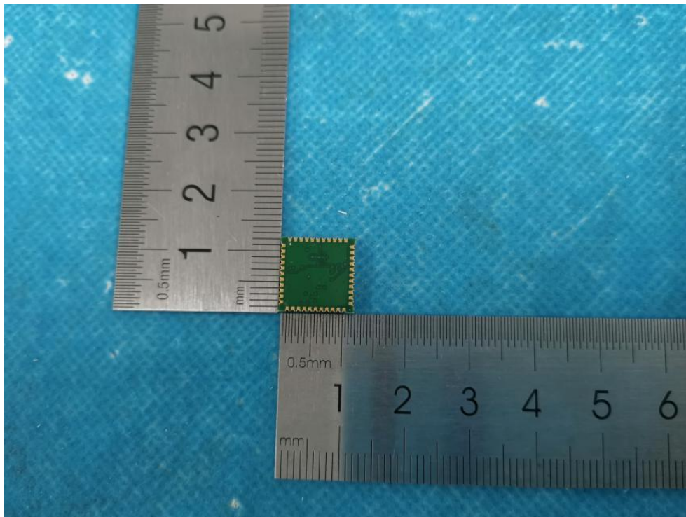
Eut Rear
