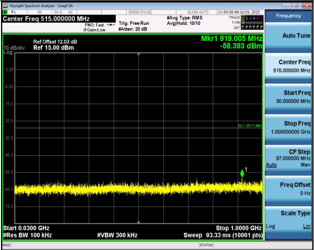
11AX20SISO-Ant1-2437-30~1000-PASS
