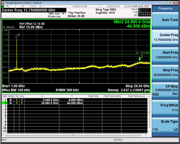
11AX40SISO-Ant1-2452-1000~26500-PASS
