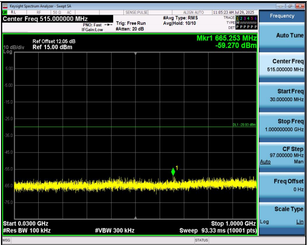
11AX20SISO-Ant1-2412-30~1000-PASS
