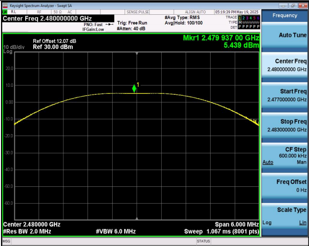
LE_2M-Ant1-2480-PASS
