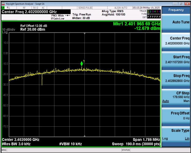
LE_2M-Ant1-2402-PASS
