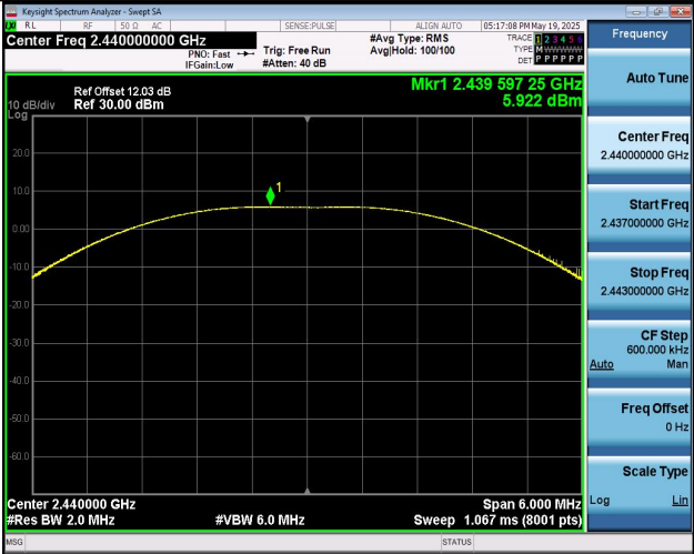
LE_2M-Ant1-2440-PASS
