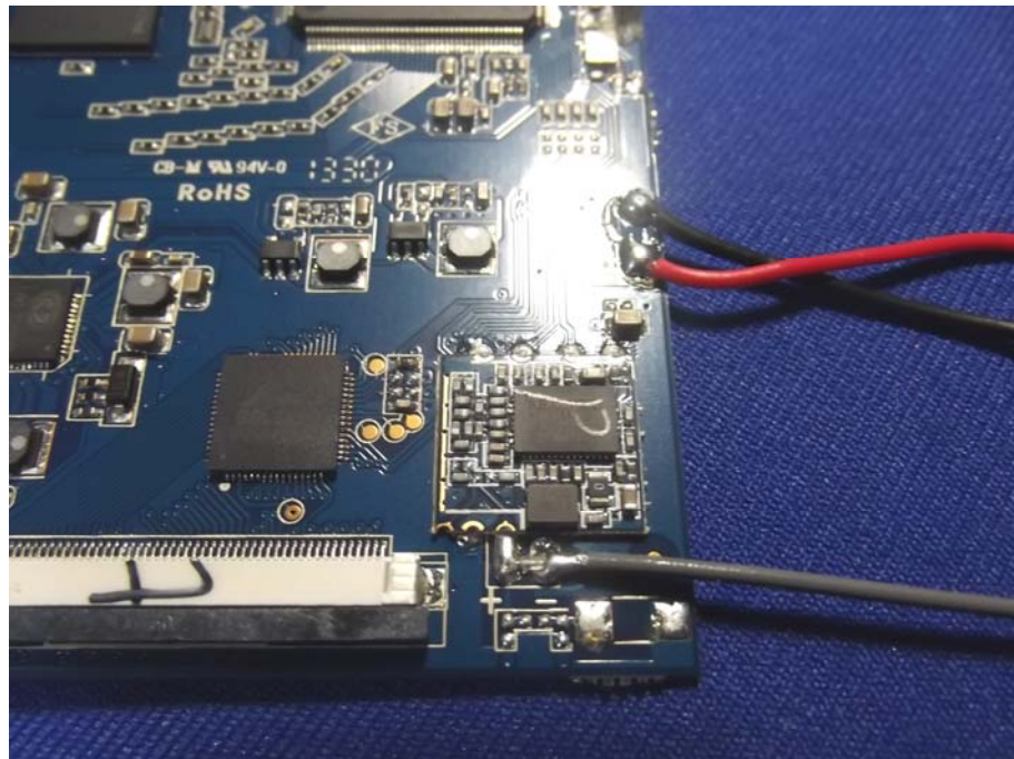
Figure 8 PCB of the WIFI Module View
