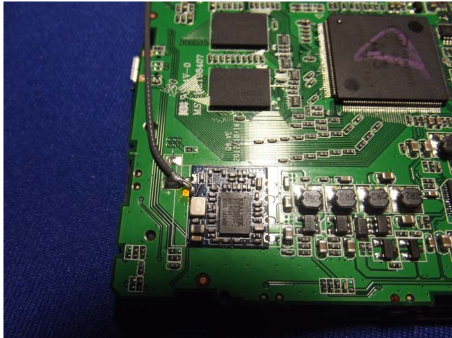
Figure 9 PCB of the BT Module View
