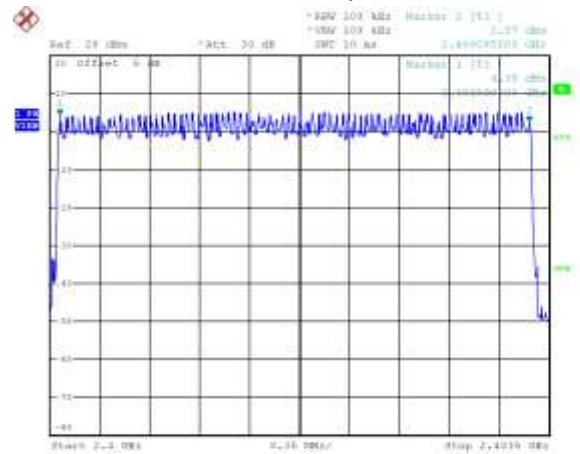
3 Mbps
