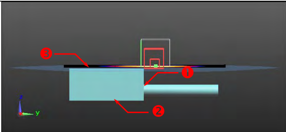
Figure 4. Body SAR Test Setup (Flat Section)
