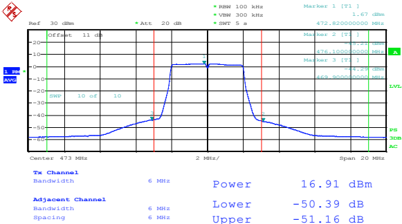
Figure 8.4-1: Adjacent channel power for low channel
