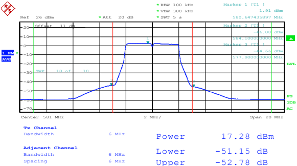
Figure 8.4-2: Adjacent channel power for mid channel
