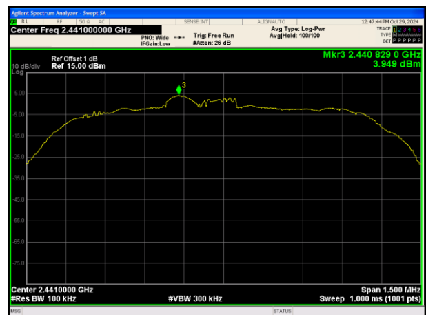
In-Band Reference Level 8DPSK_3-DH5_Channel 39
