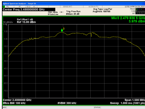
In-Band Reference Level 8DPSK_3-DH5_Channel 78
