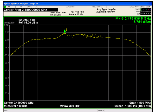
In-Band Reference Level \pi/4 DQPSK_2-DH5_Channel 78
