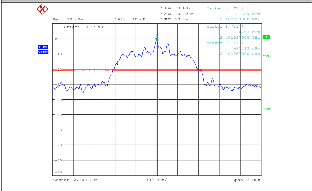
20 dB Bandwidth_2DH5_2402
