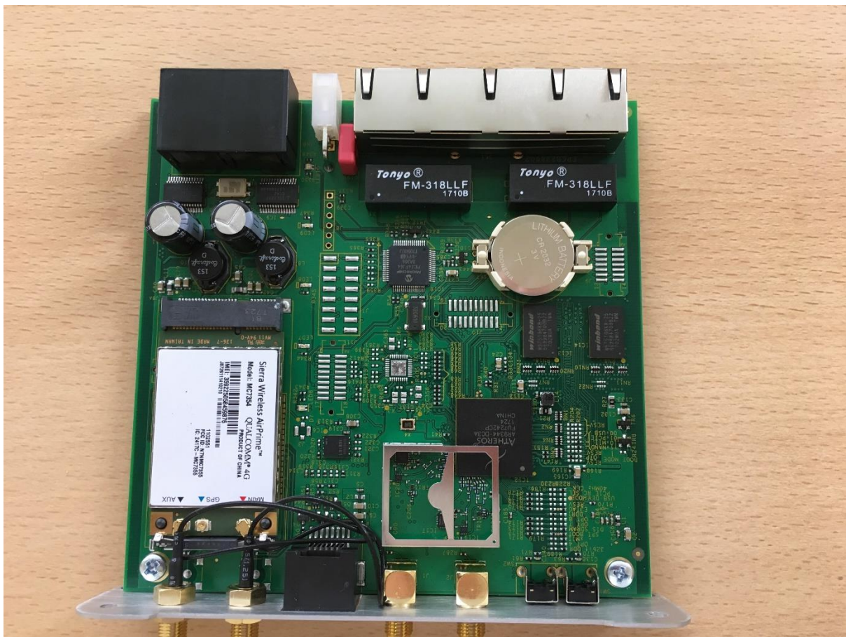
Figure 2: Hera604v4 PCB Top Wifi Screen cage fitted
