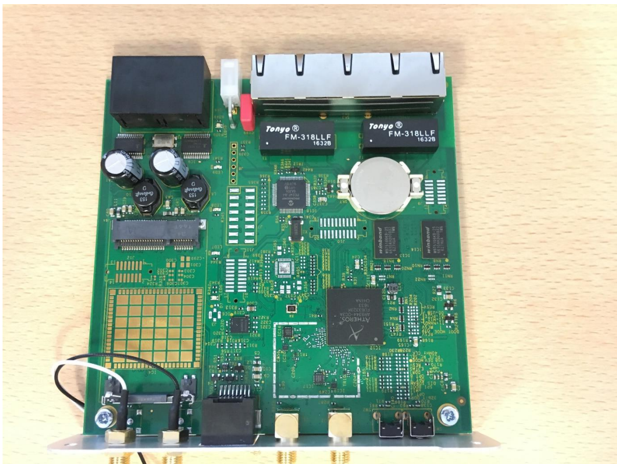
Figure 1: Hera604v4 PCB Top Cellular modem and Wifi Cage rremoved
