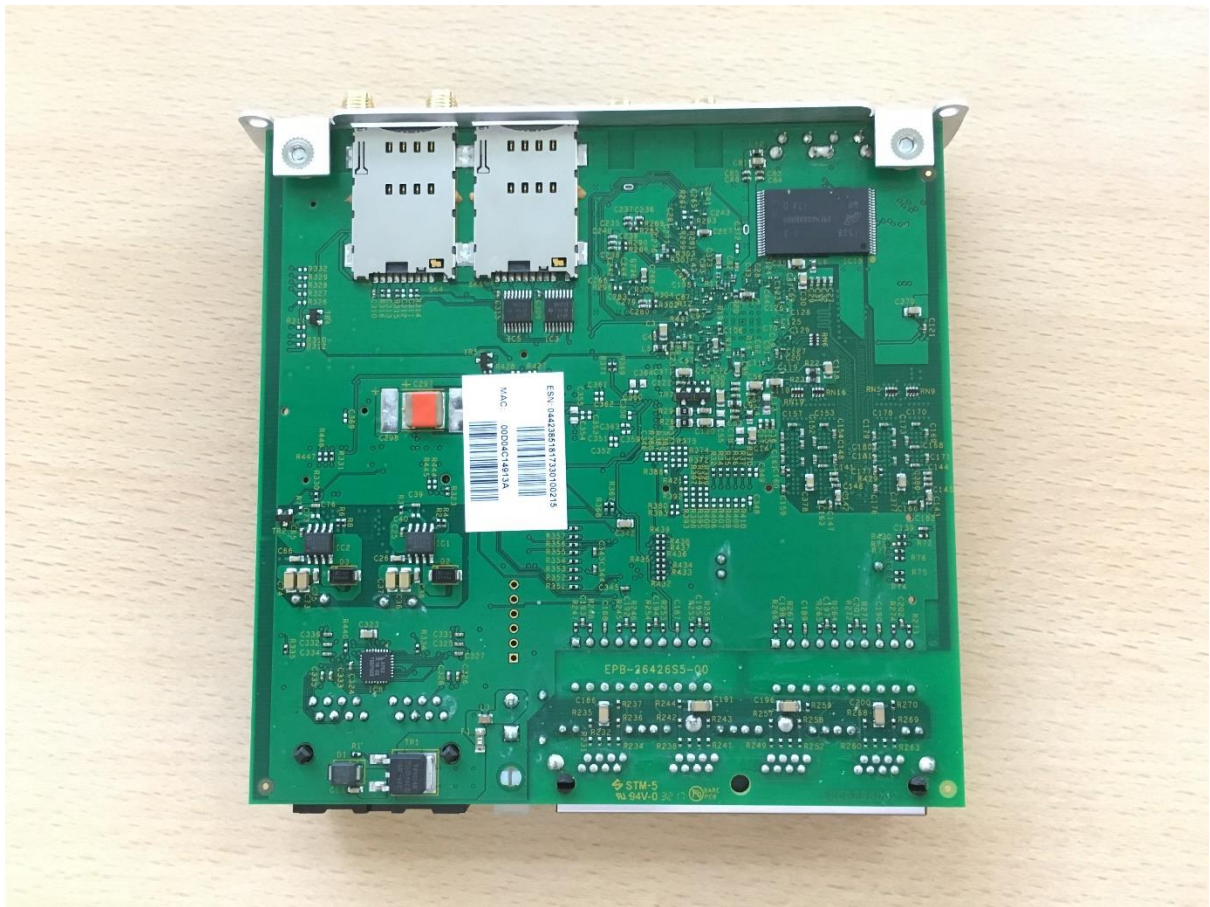
Figure 4: Hera604v4 PCB Bottom
