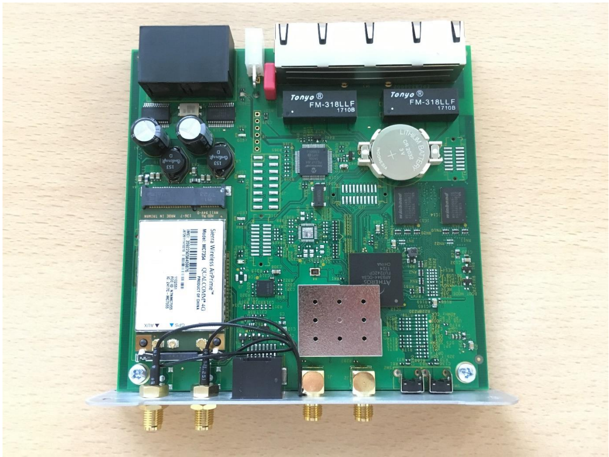
Figure 3: Hera604v4 PCB Top with WiFi Screen Fitted
