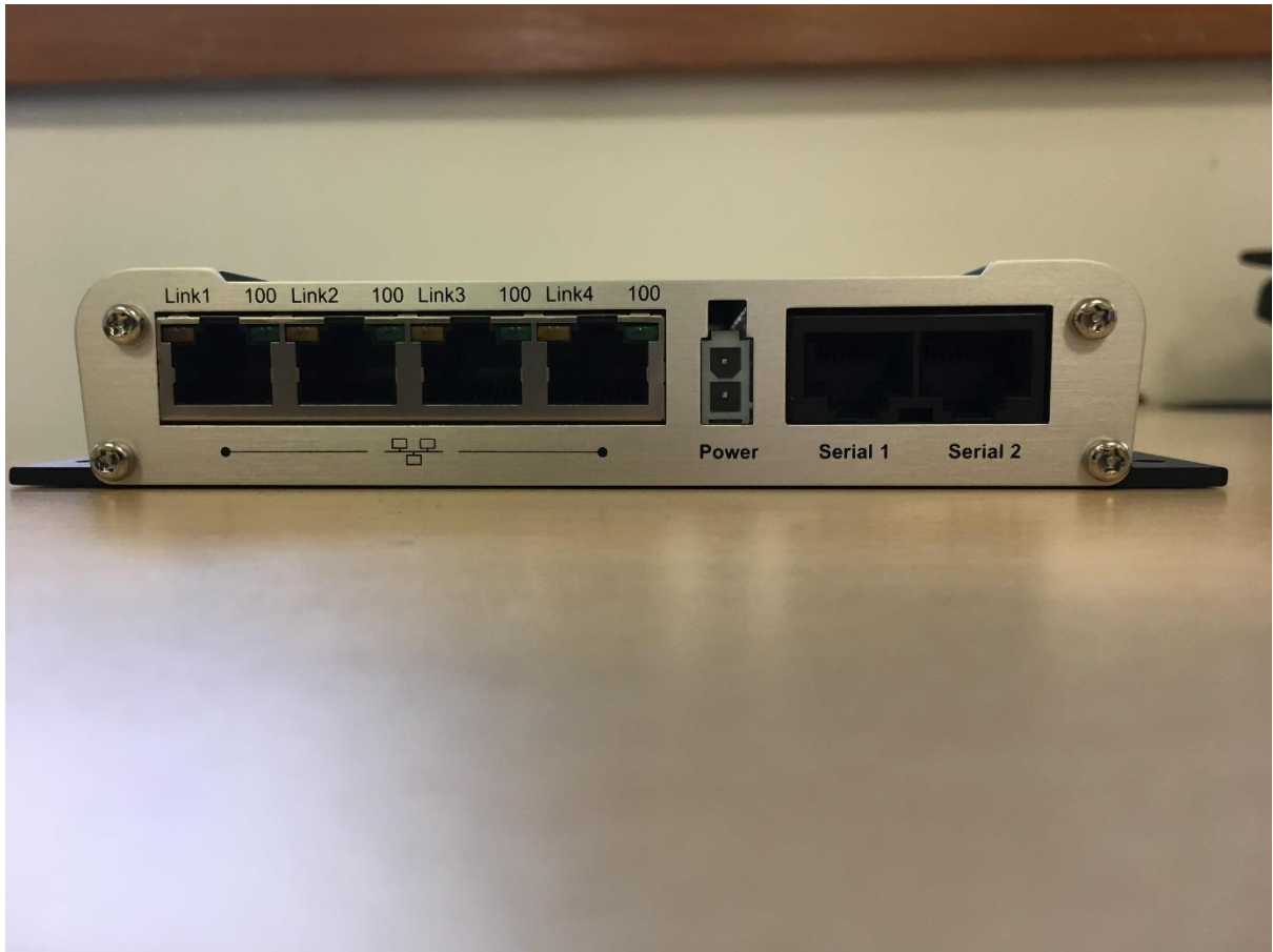
Figure 4: Hera604v4 Bottom Panel
