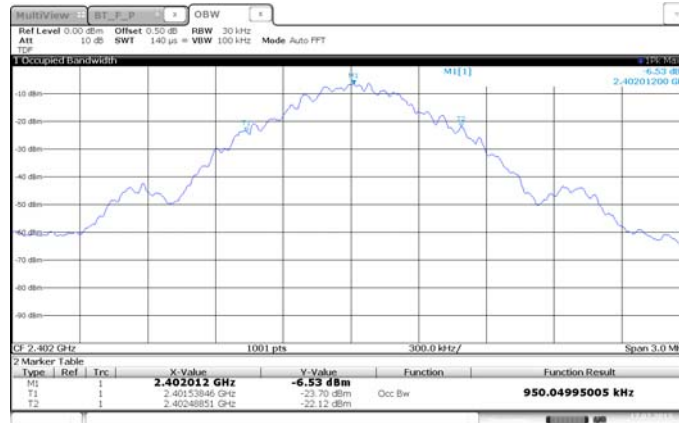
Figure 4. Plot of the Occupied Bandwidth (Conducted)
