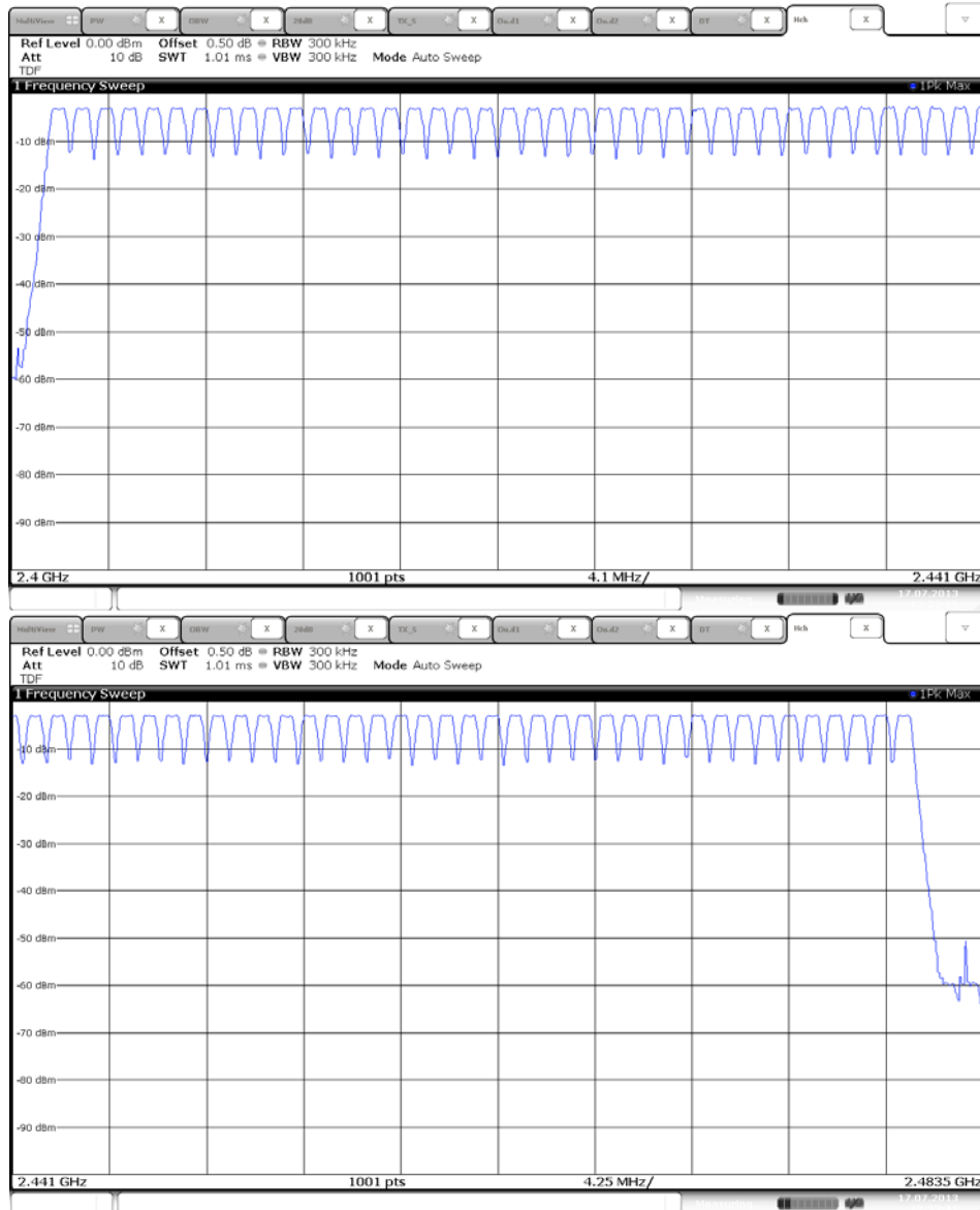
Figure 4. Plot of the Number of Hopping Channels (Conducted)
