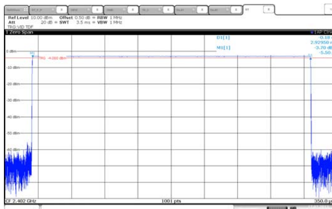
Figure 5. Plot of the Time of Occupancy (Conducted)
