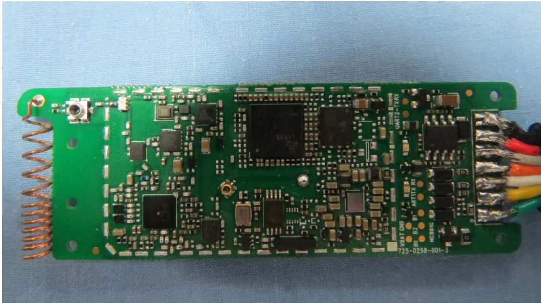
Without Shielding Case-- front side
