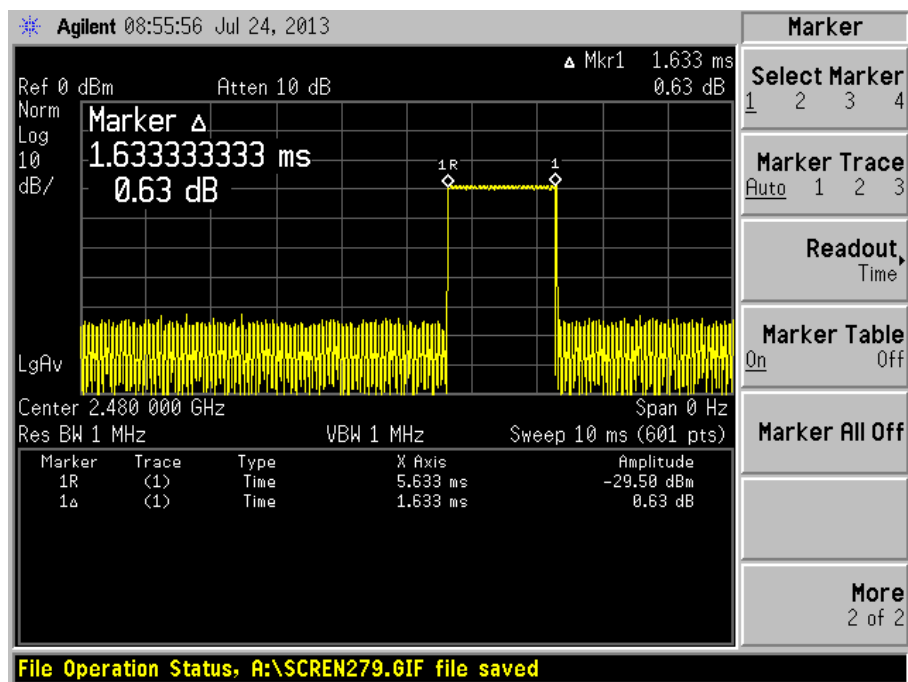
Channel 79_ 2480 MHz_DH3
