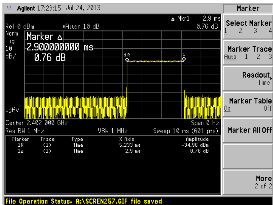
Channel 1_ 2402 MHz_DH5
