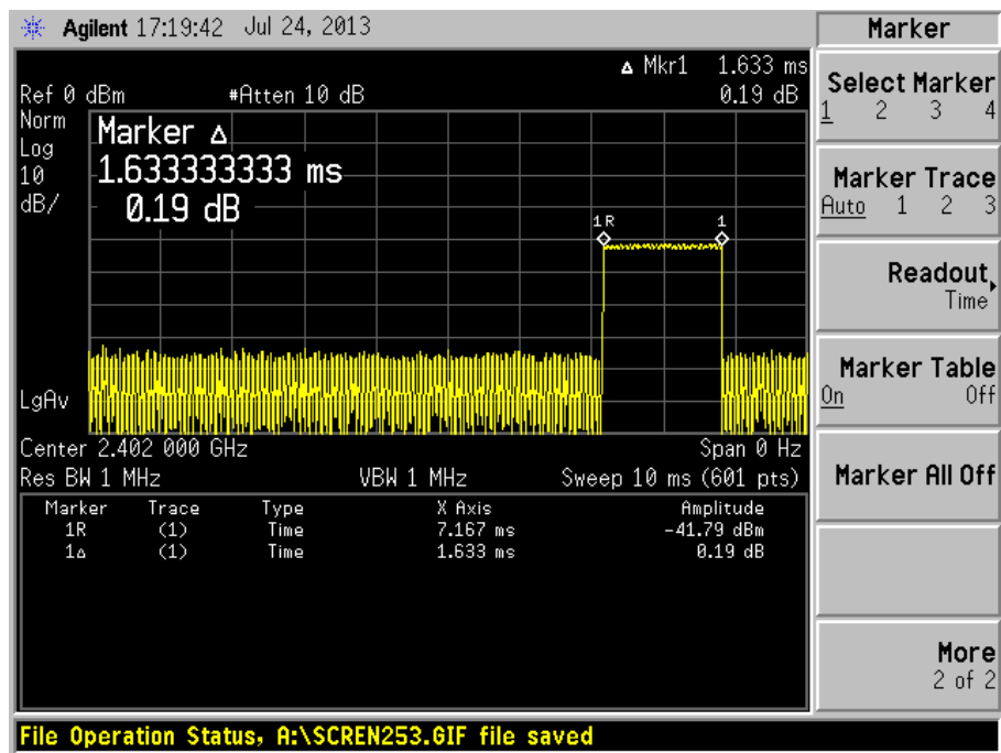
Channel 1_ 2402 MHz_DH3
