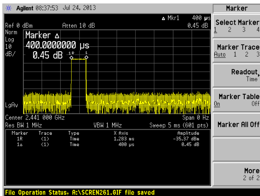
Channel 40_ 2441 MHz_DH1
