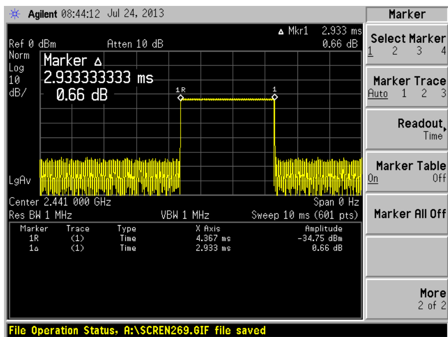
Channel 40_ 2441 MHz_DH5
