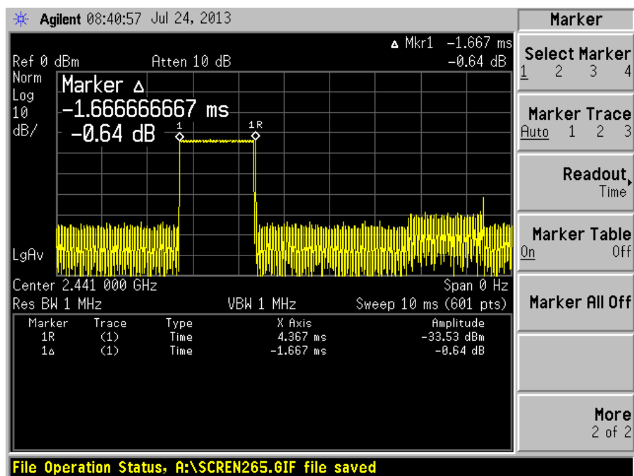
Channel 40_ 2441 MHz_DH3
