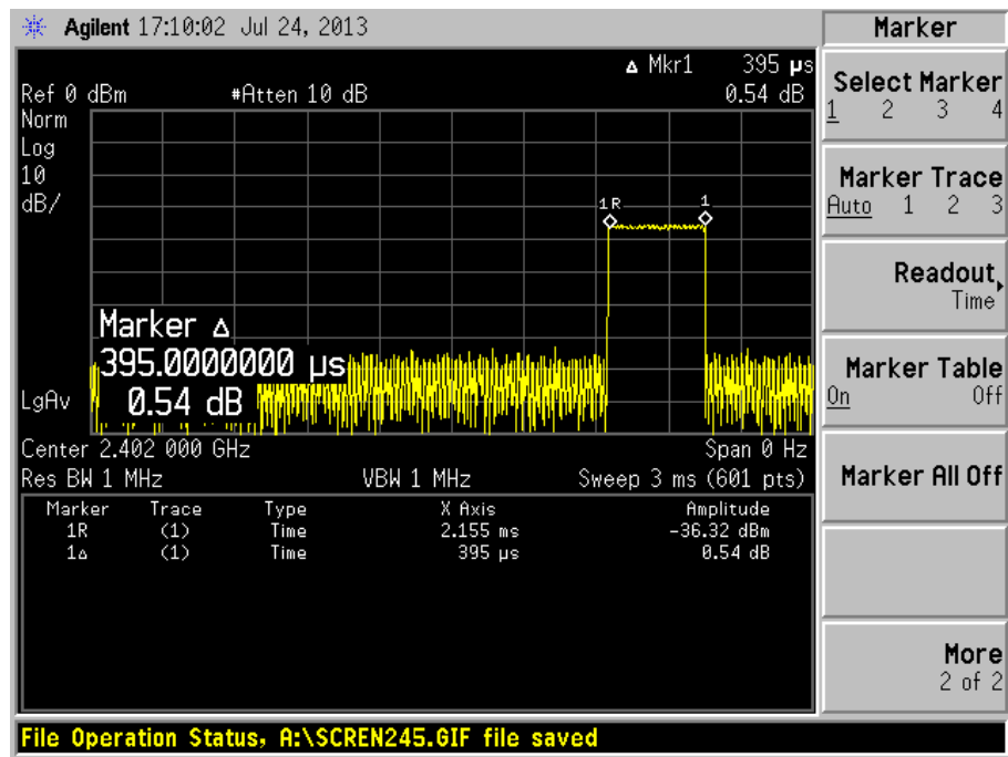
Channel 1_ 2402 MHz_DH1
