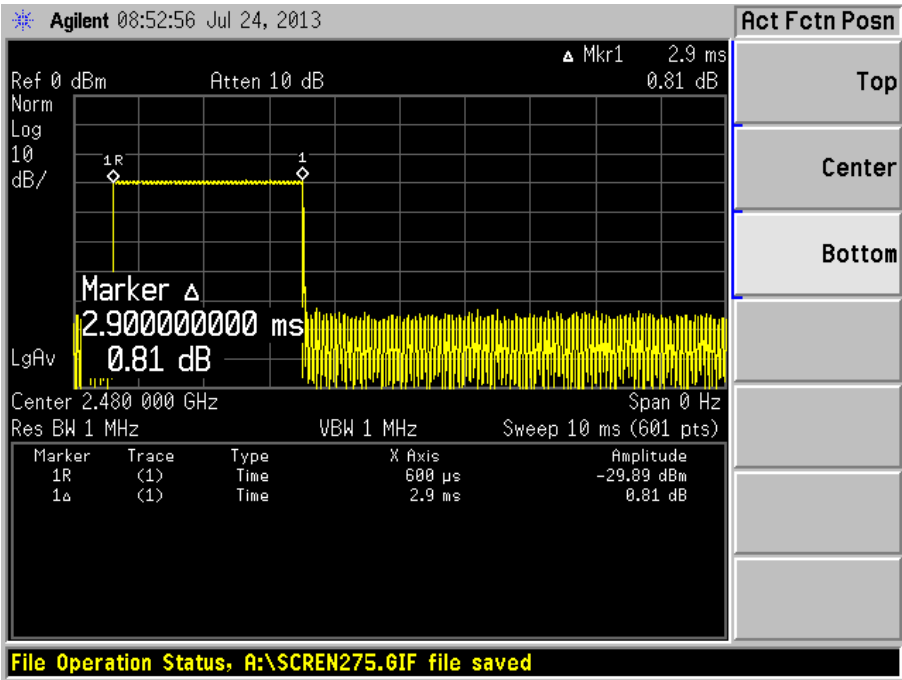
Channel 79_ 2480 MHz_DH5
