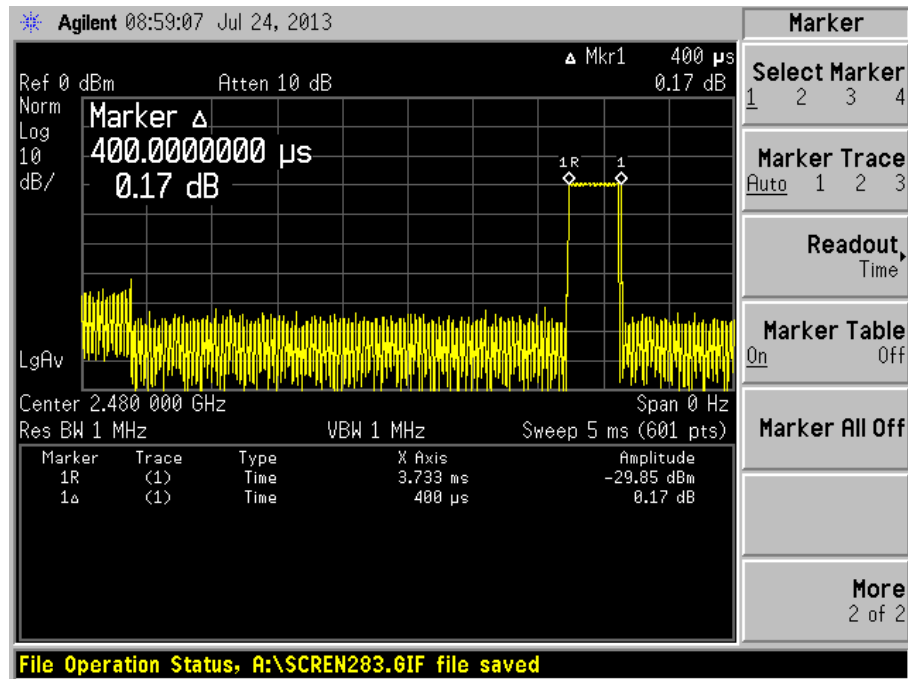
Channel 79_ 2480 MHz_DH1
