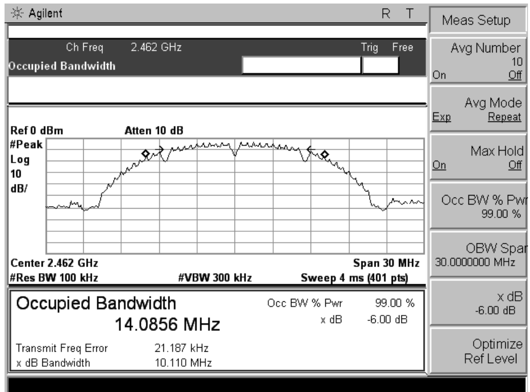
802.11g channel, 6 dB Spectrum Bandwidth &amp; 99% Occupied Bandwidth
