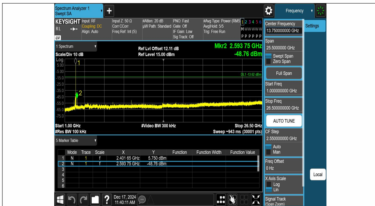
BLE_1M-Ant1-2402-1000~26500-PASS
