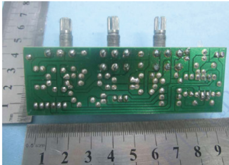
Solder Board-Component View 6
