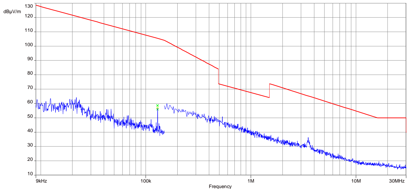
Plot 2: 9 kHz – 30 MHz; magnetic emissions; open cover
