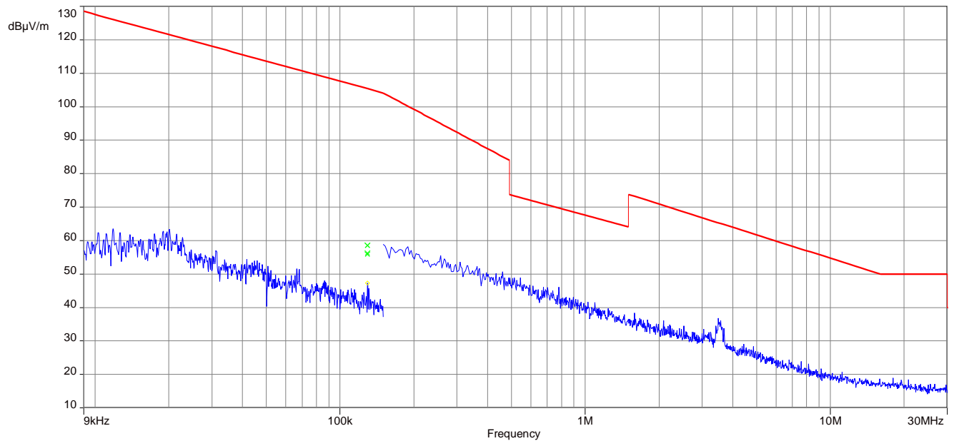
Plot 1: 9 kHz – 30 MHz; magnetic emissions; closed cover
