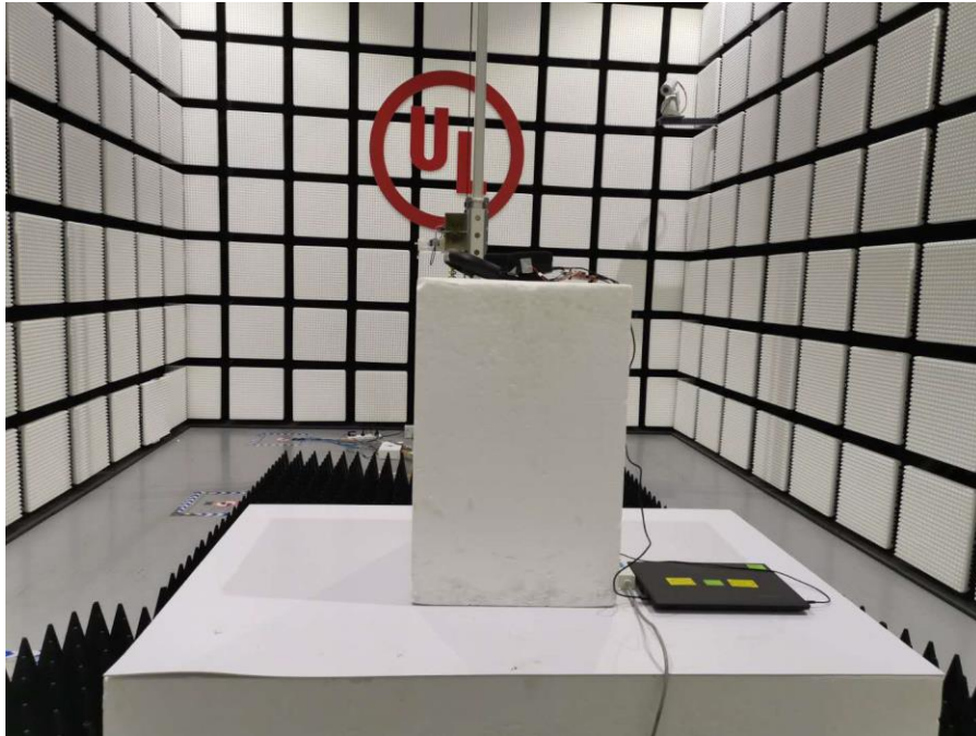
MEASUREMENT POSITION
