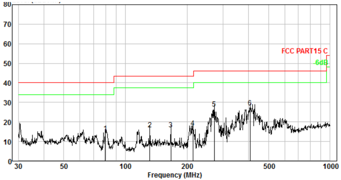
Test plot for Vertical: GFSK(2402MHz)
