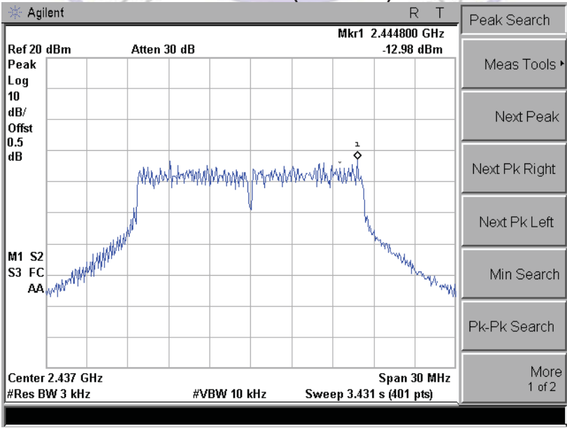
Channel 06 (2437MHz)
