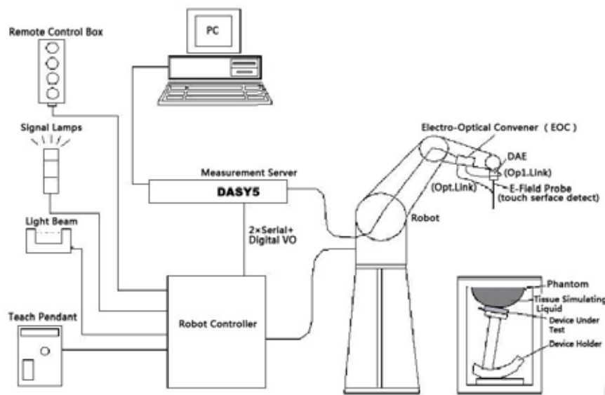
Picture 1. SAR Lab Test Measurement Set-up
