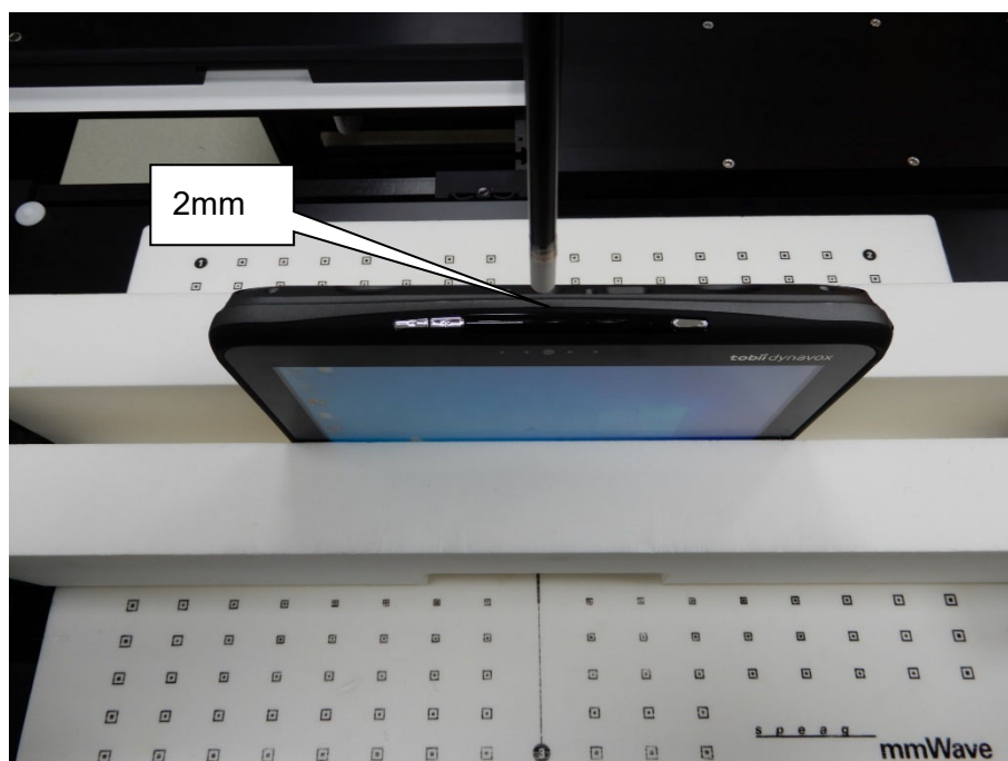
EUT PD_Top_2mm
