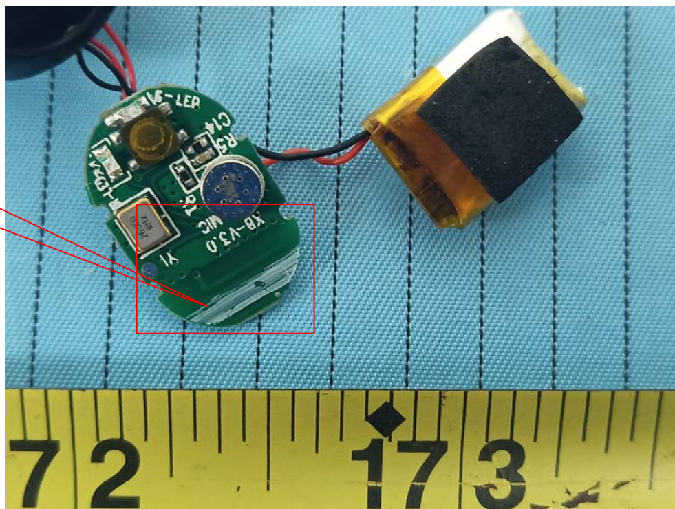
BT Antenna
