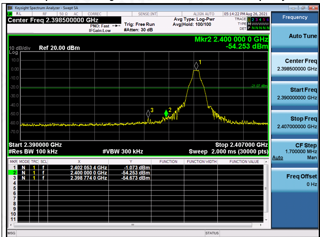
Test Graph BR ANT1 2402 1Mbps Lower Band Edge Emissions
