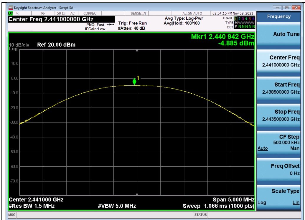
Test_Graph_BR_ANT1_2441_1Mbps_Peak Power
