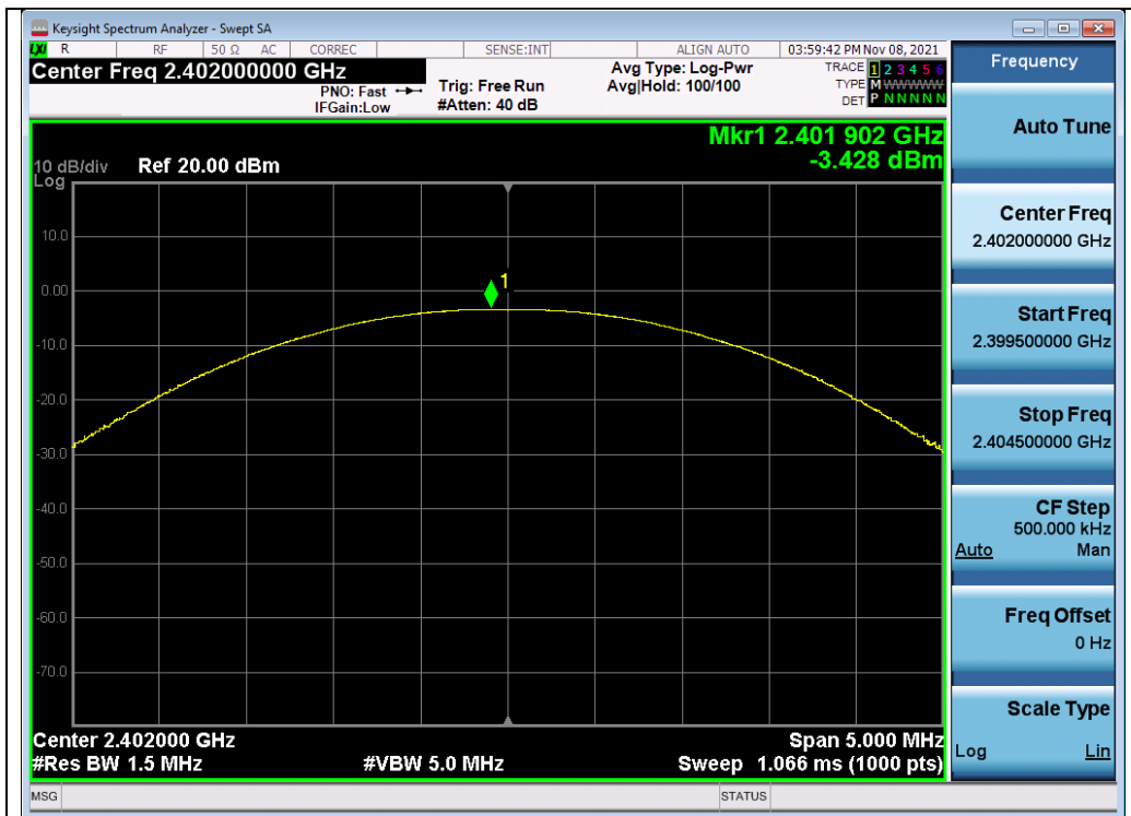
Test_Graph_EDR_ANT1_2402_2Mbps_Peak Power
