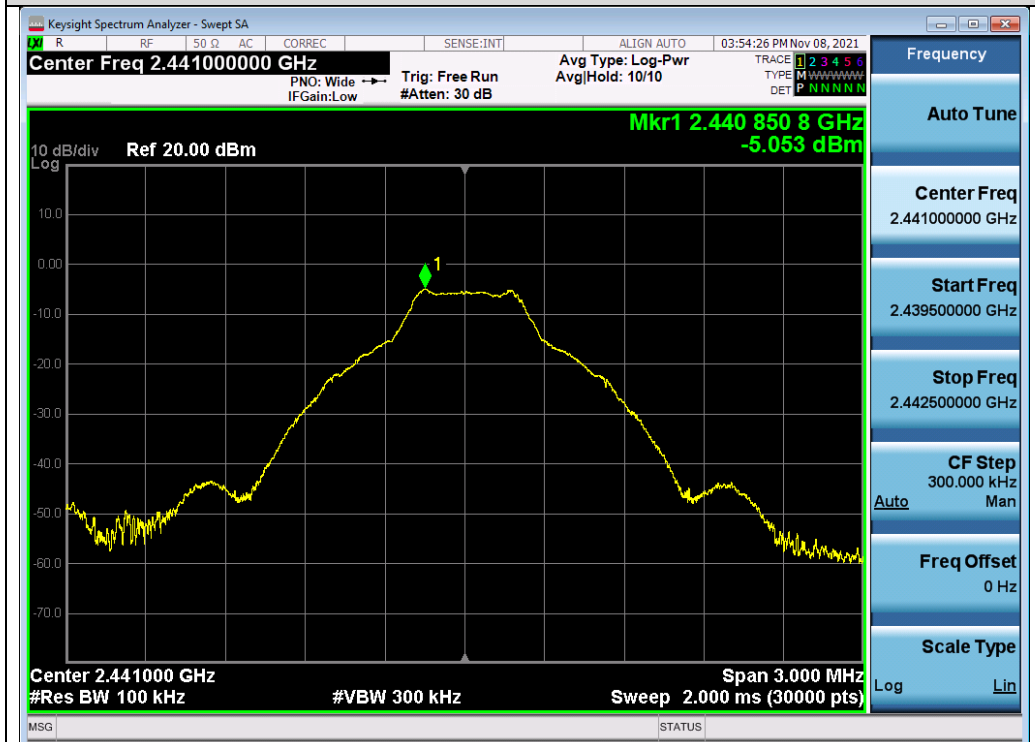
Test_Graph_BR_ANT1_2441_1Mbps_Reference Level
