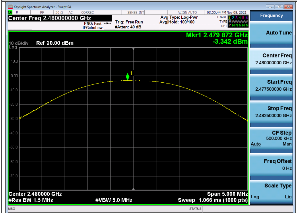
Test_Graph_BR_ANT1_2480_1Mbps_Peak Power
