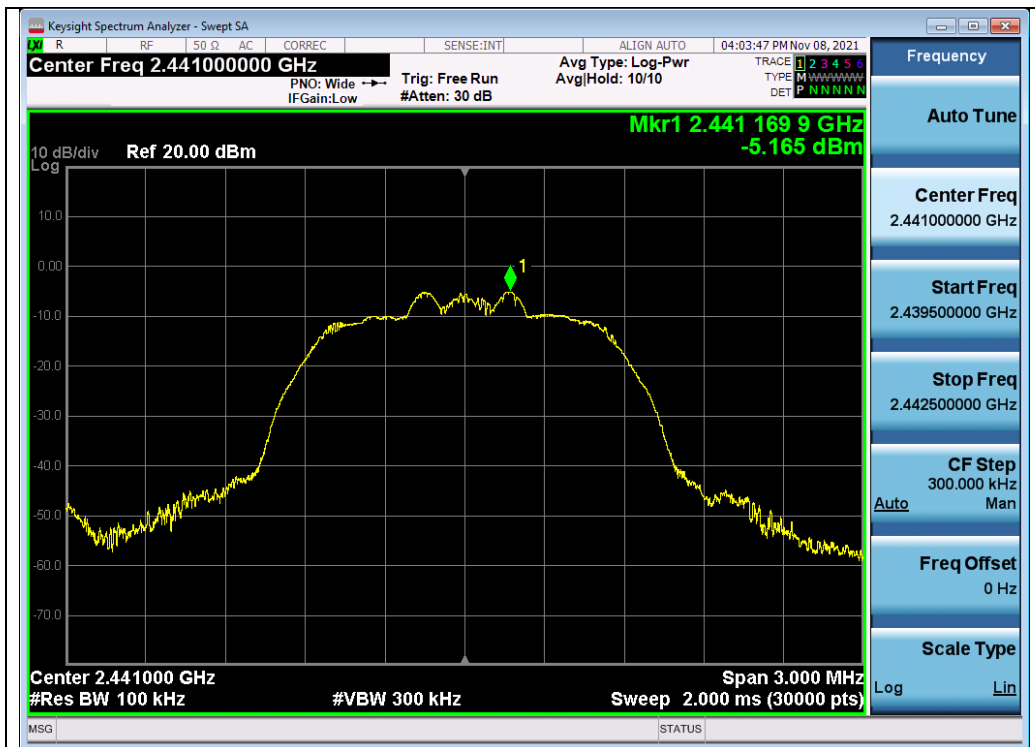
Test_Graph_EDR_ANT1_2441_2Mbps_Reference Level
