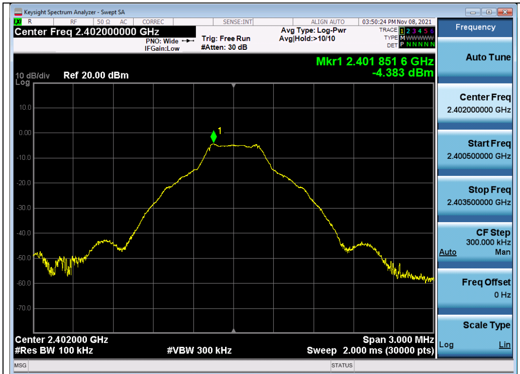
Test_Graph_BR_ANT1_2402_1Mbps_Reference Level
