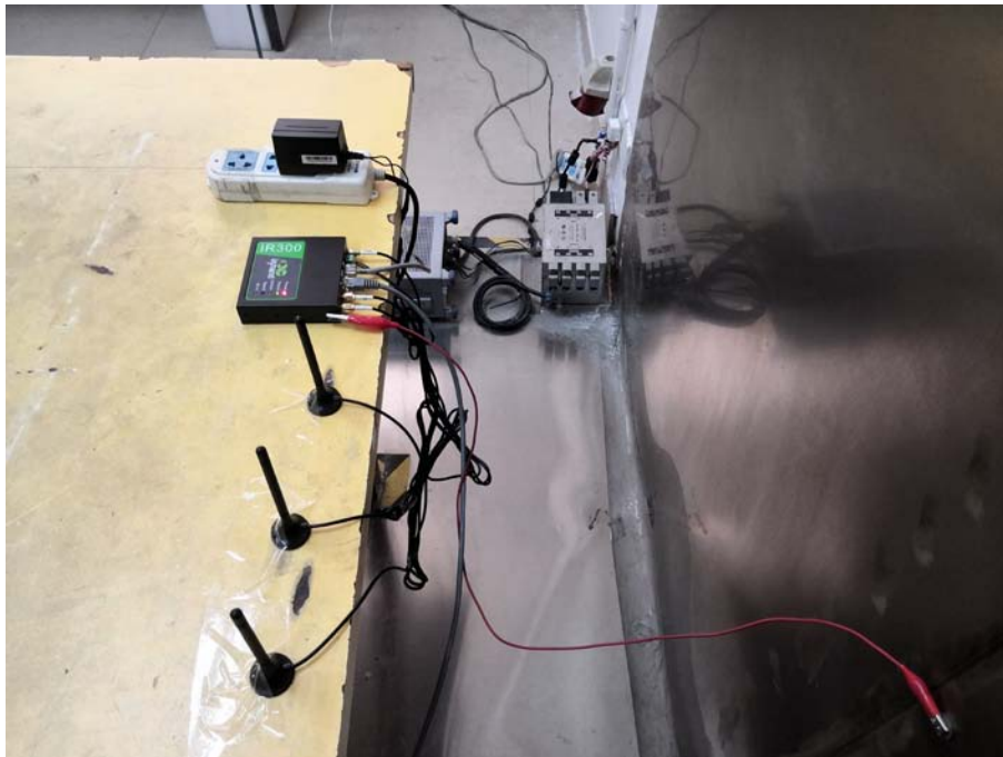
Conducted Emissions Test Setup Side View
