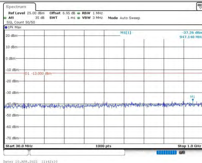
Band4-15MHz-16QAM-20325-1RB#0-Range1:30~1000MHz
