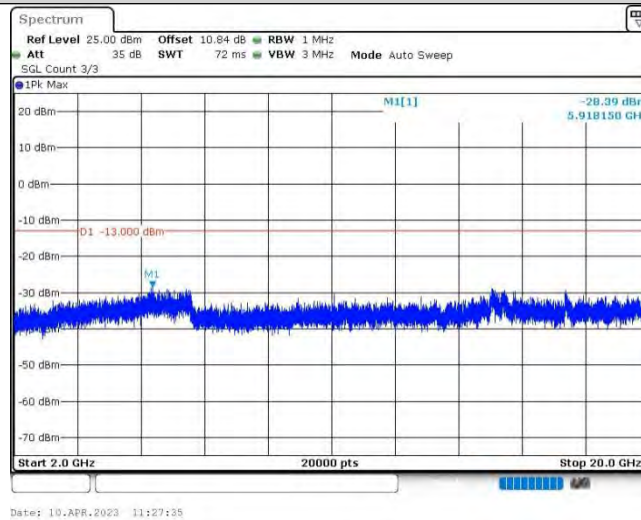
Band4-5MHz-16QAM-20175-1RB#0-Range3:2000~20000MHz
