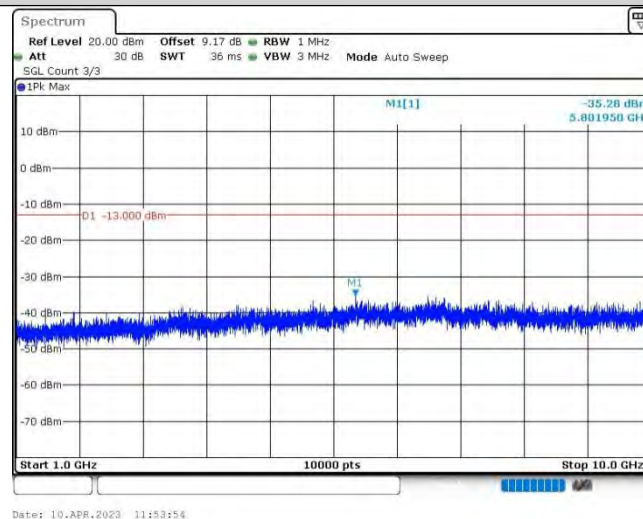
Band5-3MHz-16QAM-20525-1RB#0-Range2:1000~10000MHz
