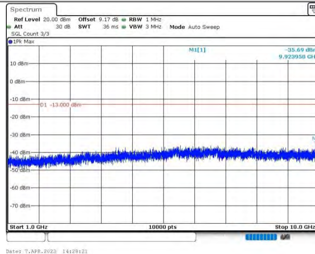
Band12-1.4MHz-QPSK-23173-1RB#0-Range2:1000~10000MHz
