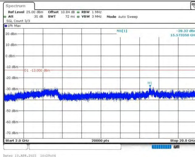
Band25-1.4MHz-16QAM-26047-1RB#0-Range3:2000~20000MHz
