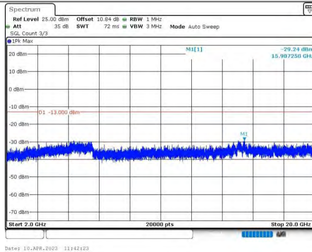
Band4-15MHz-16QAM-20325-1RB#0-Range3:2000~20000MHz
