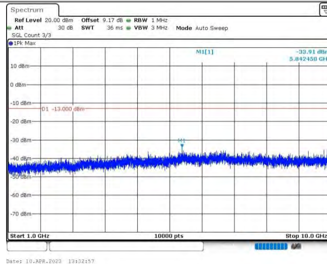
Band5-10MHz-16QAM-20600-1RB#0-Range2:1000~10000MHz
