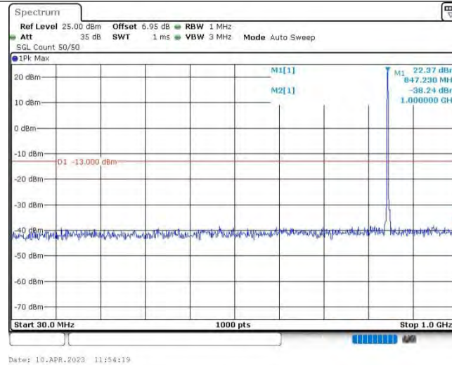
Band5-3MHz-16QAM-20635-1RB#0-Range1:30~1000MHz
