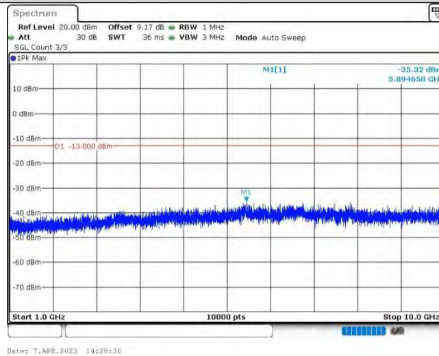
Band12-1.4MHz-16QAM-23173-1RB#0-Range2:1000~10000MHz
