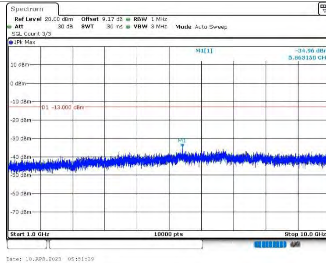
Band12-5MHz-QPSK-23035-1RB#0-Range2:1000~10000MHz
