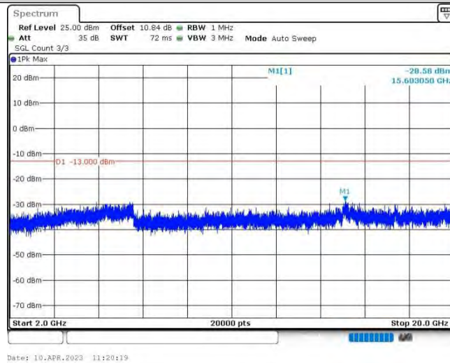
Band4-3MHz-16QAM-19965-1RB#0-Range3:2000~20000MHz
