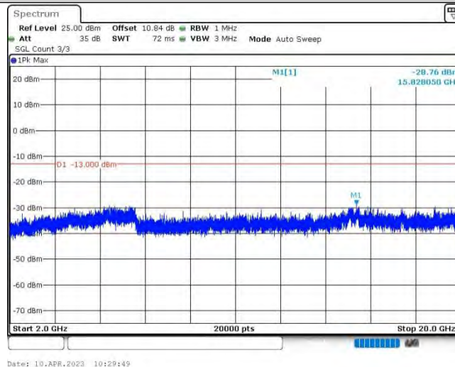
Band25-1.4MHz-16QAM-26365-1RB#0-Range3:2000~20000MHz
