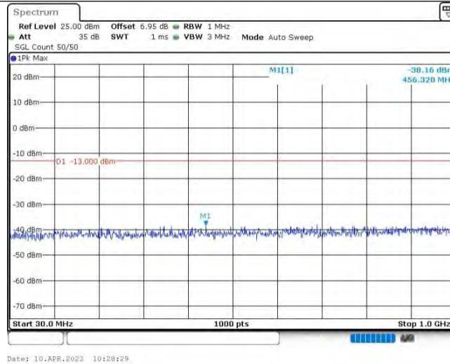
Band25-1.4MHz-QPSK-26047-1RB#0-Range1:30~1000MHz
