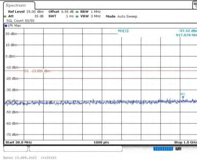
Band25-1.4MHz-16QAM-26047-1RB#0-Range1:30~1000MHz
