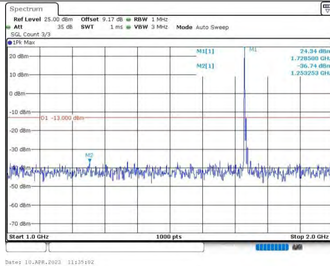
Band4-10MHz-16QAM-20175-1RB#0-Range2:1000~2000MHz
