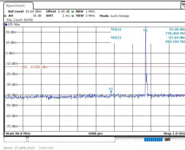
Band13-10MHz-16QAM-23230-1RB#0-Range1:30~1000MHz
