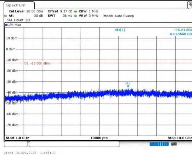
Band5-5MHz-16QAM-20425-1RB#0-Range2:1000~10000MHz
