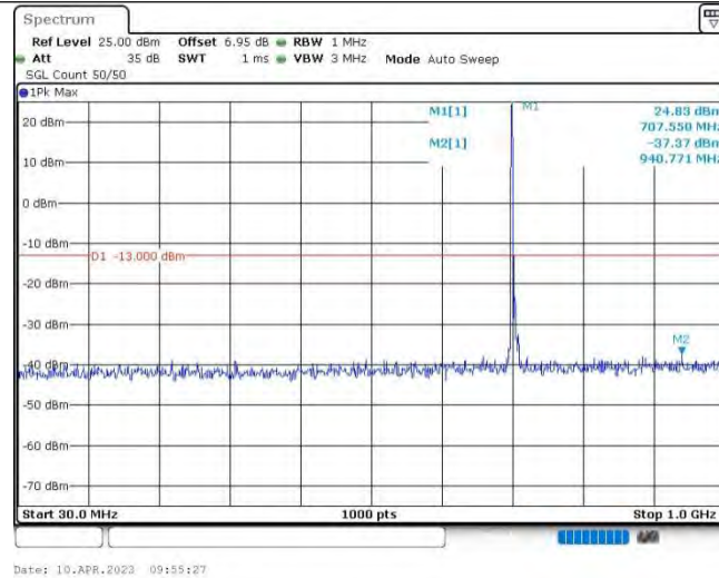
Band12-10MHz-16QAM-23130-1RB#0-Range1:30~1000MHz
