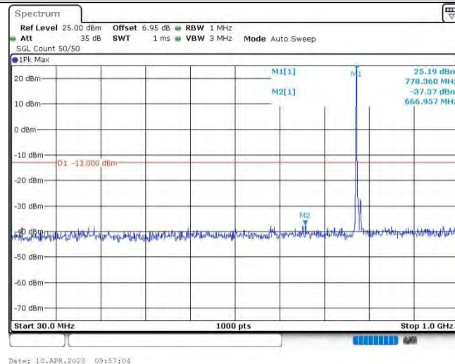
Band13-5MHz-QPSK-23205-1RB#0-Range1:30~1000MHz
