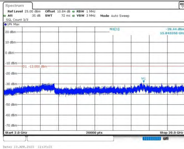
Band4-10MHz-QPSK-20350-1RB#0-Range3:2000~20000MHz
