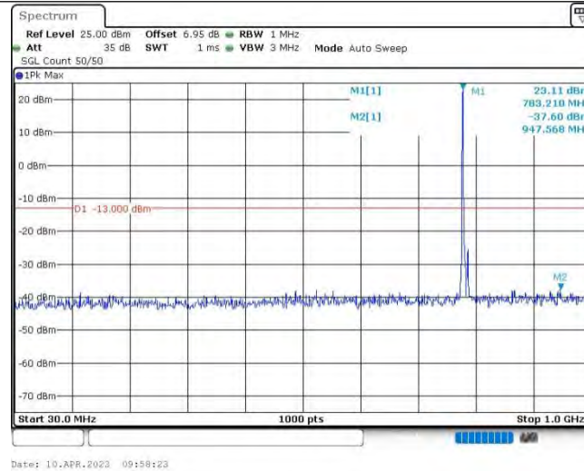
Band13-5MHz-16QAM-23255-1RB#0-Range1:30~1000MHz
