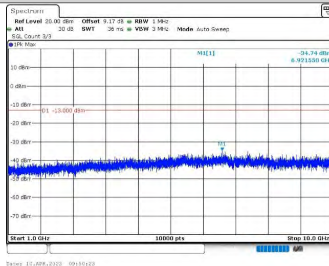
Band12-3MHz-QPSK-23095-1RB#0-Range2:1000~10000MHz
