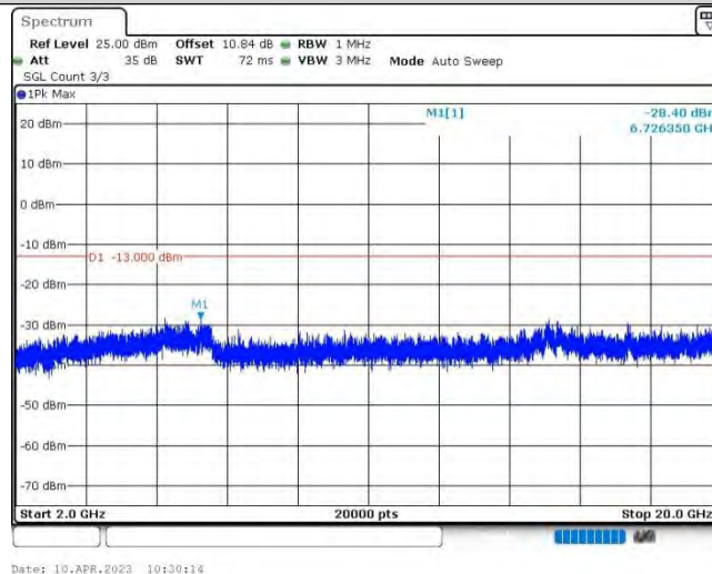
Band25-1.4MHz-QPSK-26683-1RB#0-Range3:2000~20000MHz
