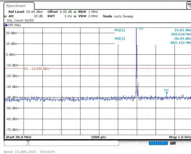
Band12-5MHz-QPSK-23095-1RB#0-Range1:30~1000MHz
