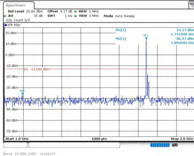
Band4-15MHz-16QAM-20325-1RB#0-Range2:1000~2000MHz
