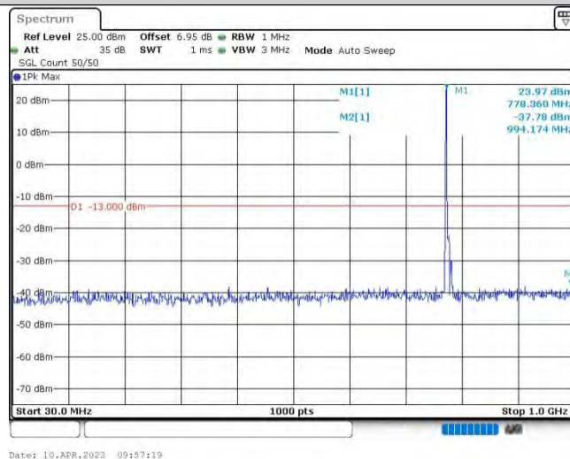
Band13-5MHz-16QAM-23205-1RB#0-Range1:30~1000MHz
