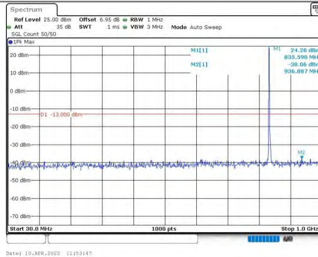
Band5-3MHz-16QAM-20525-1RB#0-Range1:30~1000MHz
