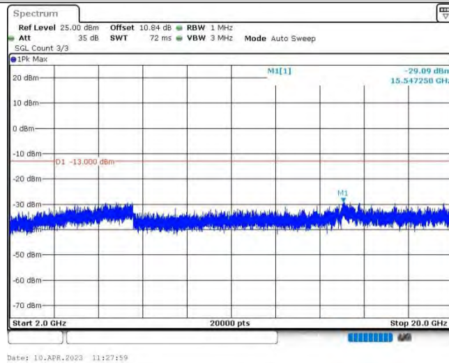
Band4-5MHz-QPSK-20375-1RB#0-Range3:2000~20000MHz
