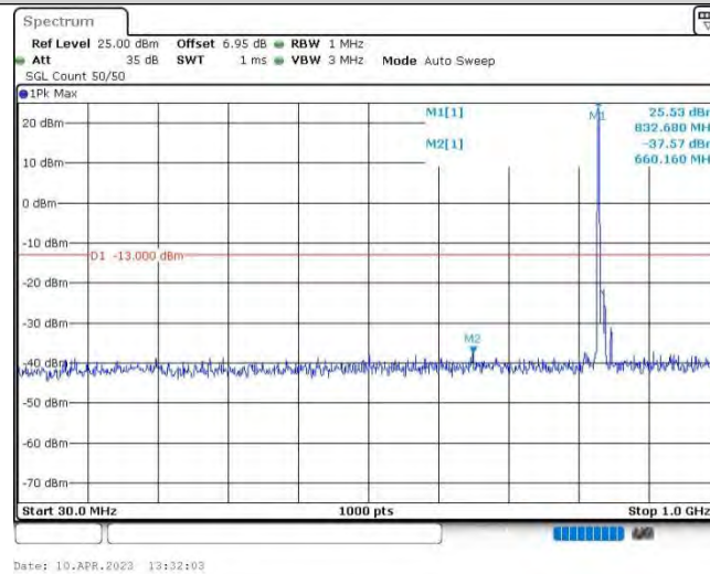
Band5-10MHz-QPSK-20525-1RB#0-Range1:30~1000MHz
