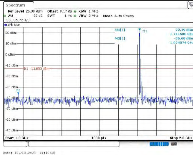
Band4-15MHz-16QAM-20025-1RB#0-Range2:1000~2000MHz
