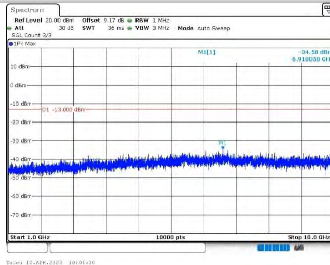
Band13-10MHz-16QAM-23230-1RB#0-Range2:1000~10000MHz
