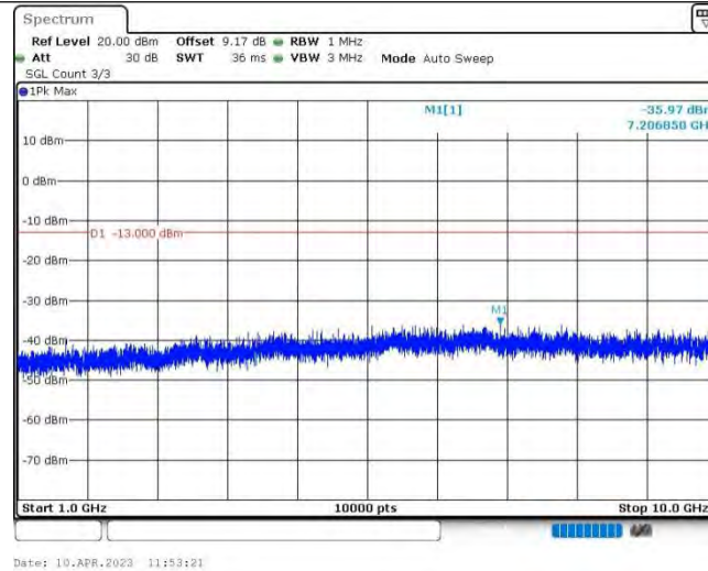
Band5-3MHz-16QAM-20415-1RB#0-Range2:1000~10000MHz
