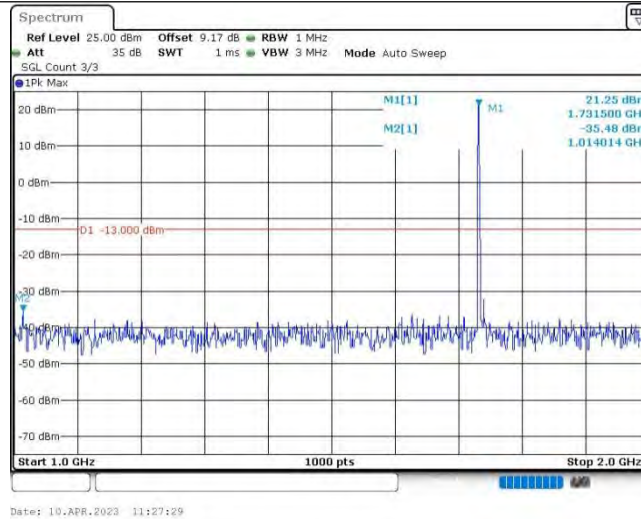
Band4-5MHz-16QAM-20175-1RB#0-Range2:1000~2000MHz
