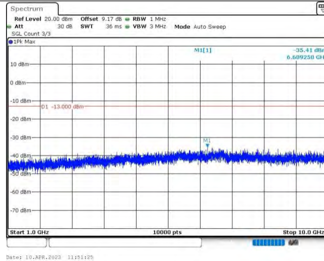
Band5-1.4MHz-16QAM-20407-1RB#0-Range2:1000~10000MHz
