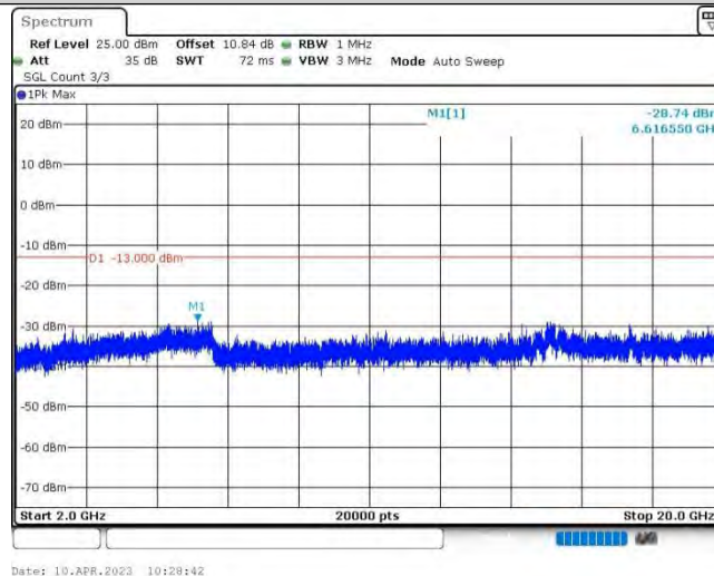
Band25-1.4MHz-QPSK-26047-1RB#0-Range3:2000~20000MHz
