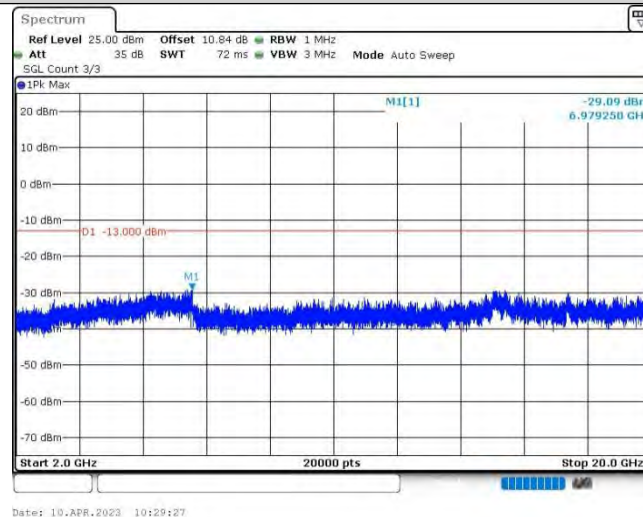
Band25-1.4MHz-QPSK-26365-1RB#0-Range3:2000~20000MHz
