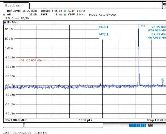
Band5-5MHz-16QAM-20425-1RB#0-Range1:30~1000MHz
