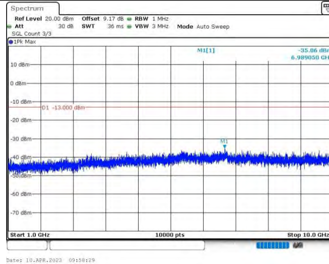
Band13-5MHz-16QAM-23255-1RB#0-Range2:1000~10000MHz
