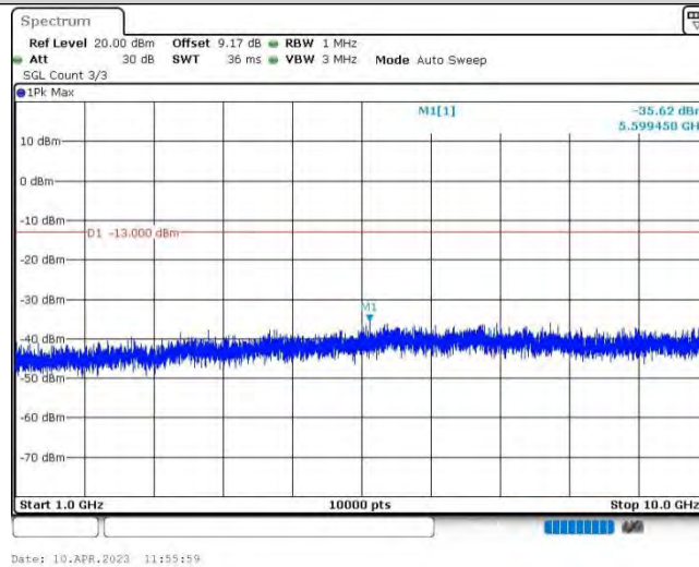
Band5-5MHz-QPSK-20625-1RB#0-Range2:1000~10000MHz
