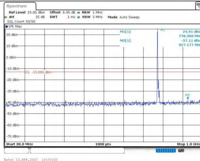
Band13-10MHz-QPSK-23230-1RB#0-Range1:30~1000MHz
