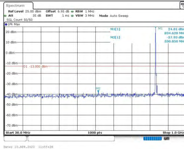
Band5-5MHz-16QAM-20525-1RB#0-Range1:30~1000MHz
