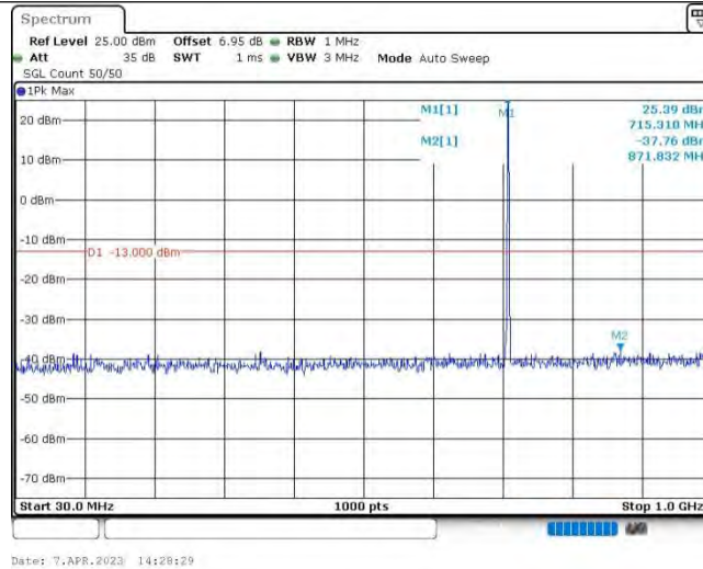
Band12-1.4MHz-16QAM-23173-1RB#0-Range1:30~1000MHz
