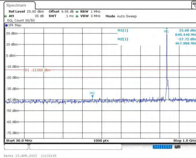
Band5-10MHz-QPSK-20600-1RB#0-Range1:30~1000MHz
