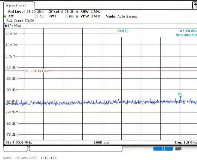
Band25-1.4MHz-16QAM-26365-1RB#0-Range1:30~1000MHz
