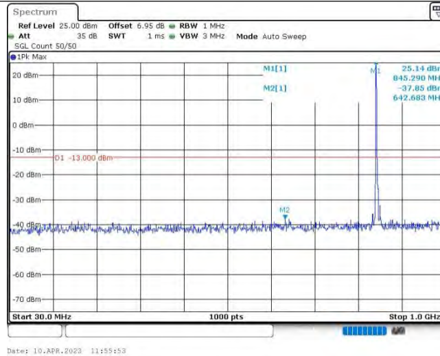
Band5-5MHz-QPSK-20625-1RB#0-Range1:30~1000MHz
