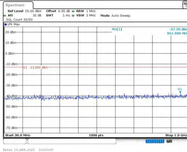
Band25-1.4MHz-QPSK-26683-1RB#0-Range1:30~1000MHz
