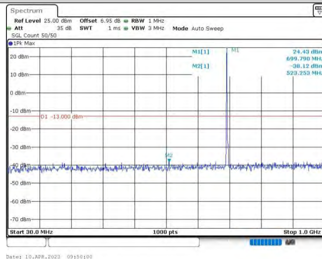
Band12-3MHz-16QAM-23025-1RB#0-Range1:30~1000MHz
