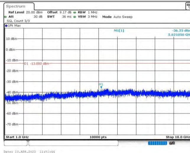
Band5-1.4MHz-QPSK-20525-1RB#0-Range2:1000~10000MHz
