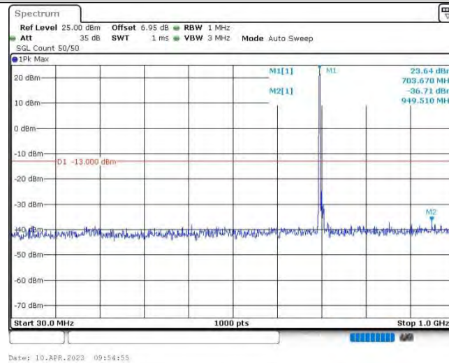
Band12-10MHz-16QAM-23095-1RB#0-Range1:30~1000MHz
