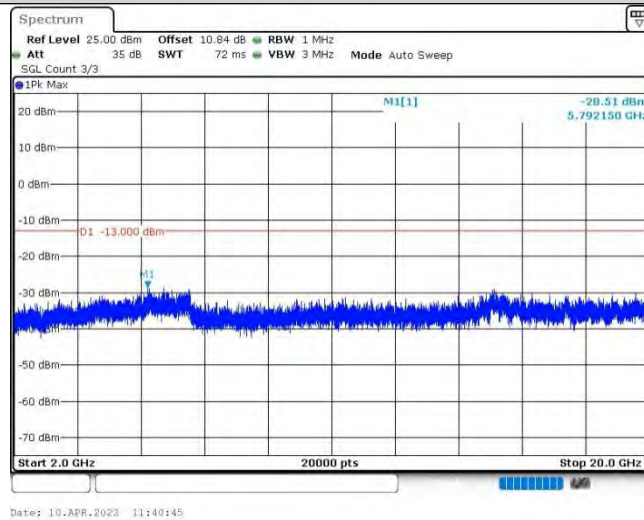
Band4-15MHz-16QAM-20025-1RB#0-Range3:2000~20000MHz
