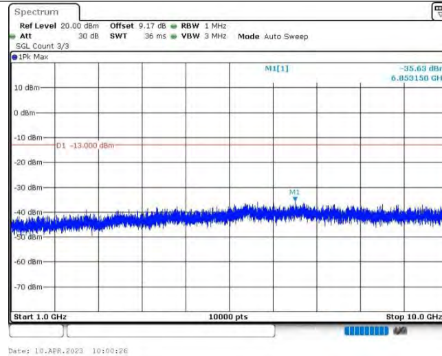
Band13-10MHz-QPSK-23230-1RB#0-Range2:1000~10000MHz
