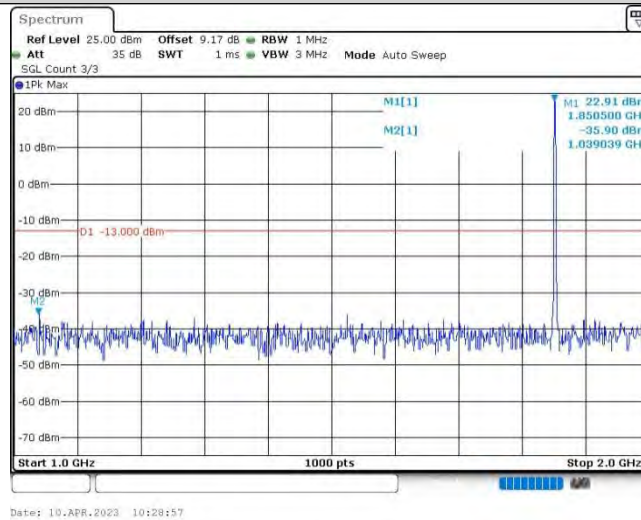
Band25-1.4MHz-16QAM-26047-1RB#0-Range2:1000~2000MHz
