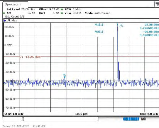
Band4-15MHz-16QAM-20175-1RB#0-Range2:1000~2000MHz
