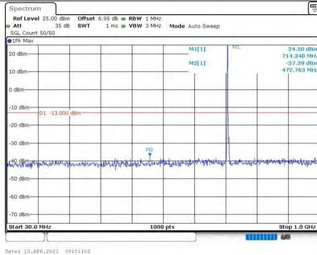
Band12-3MHz-16QAM-23165-1RB#0-Range1:30~1000MHz
