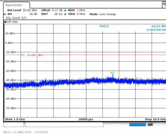
Band5-3MHz-16QAM-20635-1RB#0-Range2:1000~10000MHz
