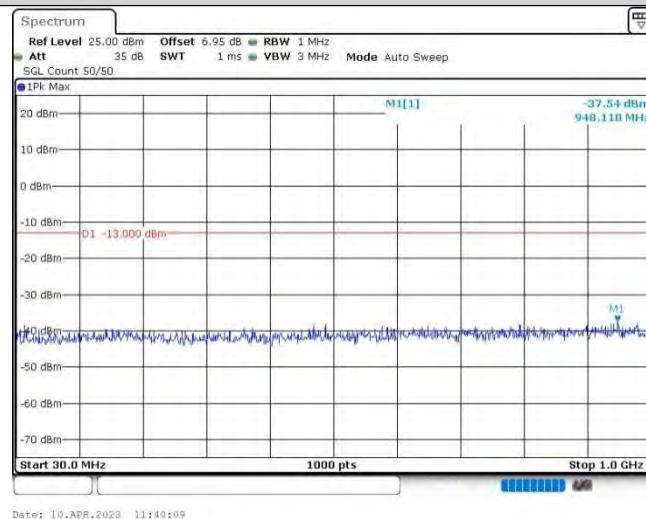
Band4-15MHz-QPSK-20025-1RB#0-Range1:30~1000MHz
