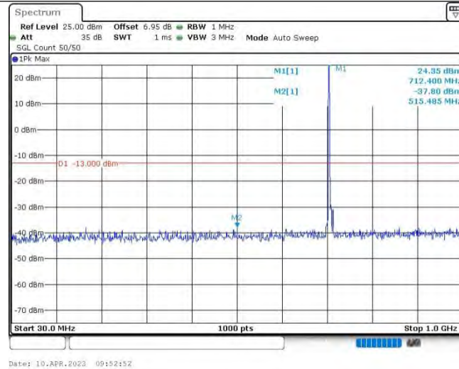
Band12-5MHz-16QAM-23155-1RB#0-Range1:30~1000MHz
