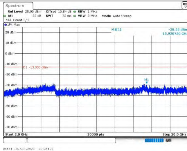
Band4-10MHz-16QAM-20175-1RB#0-Range3:2000~20000MHz
