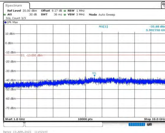
Band5-1.4MHz-16QAM-20525-1RB#0-Range2:1000~10000MHz
