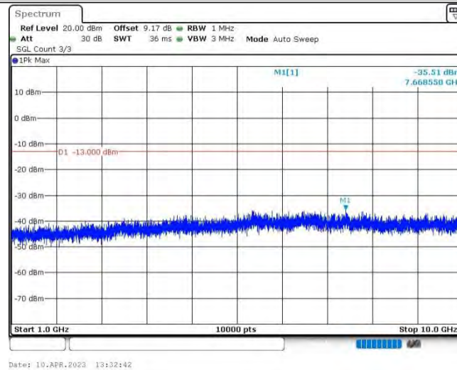
Band5-10MHz-QPSK-20600-1RB#0-Range2:1000~10000MHz
