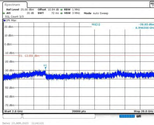
Band4-15MHz-16QAM-20175-1RB#0-Range3:2000~20000MHz
