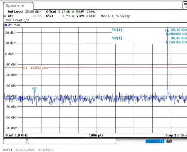
Band25-1.4MHz-16QAM-26365-1RB#0-Range2:1000~2000MHz
