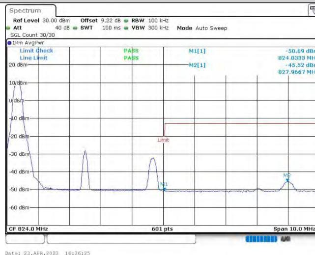
Band26@90-5MHz-16QAM-26765-1RB#0
