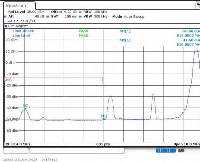
Band26@90-5MHz-QPSK-26715-1RB#24
