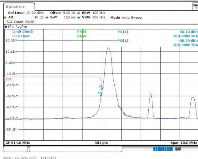
Band26@90-5MHz-QPSK-26715-1RB#0
