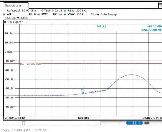
Band5-10MHz-QPSK-20450-1RB#49
