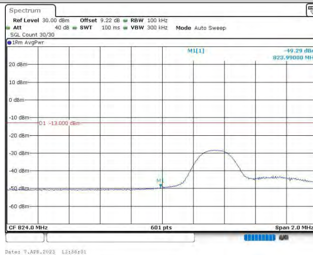
Band5-5MHz-QPSK-20425-1RB#24
