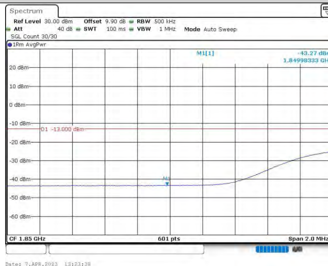
Band25-20MHz-16QAM-26140-1RB#99
