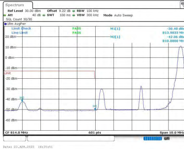
Band26@90-5MHz-16QAM-26715-1RB#24
