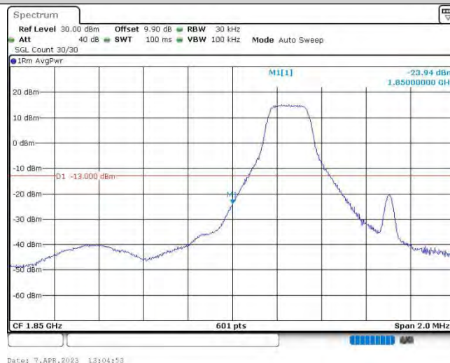
Band25-1.4MHz-QPSK-26047-1RB#0
