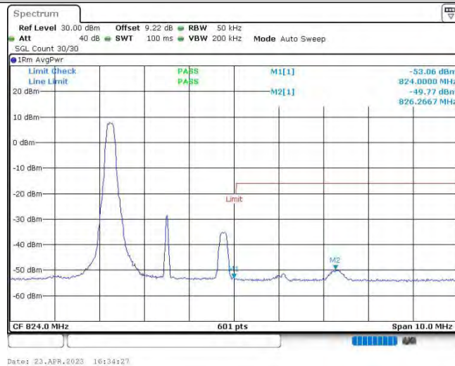
Band26@90-3MHz-16QAM-26775-1RB#0
