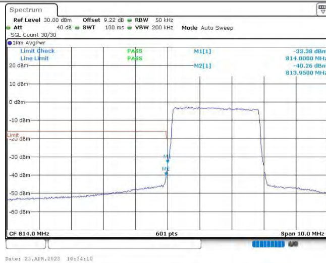
Band26@90-3MHz-16QAM-26705-15RB#0
