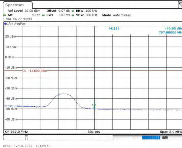
Band13-5MHz-16QAM-23255-1RB#0
