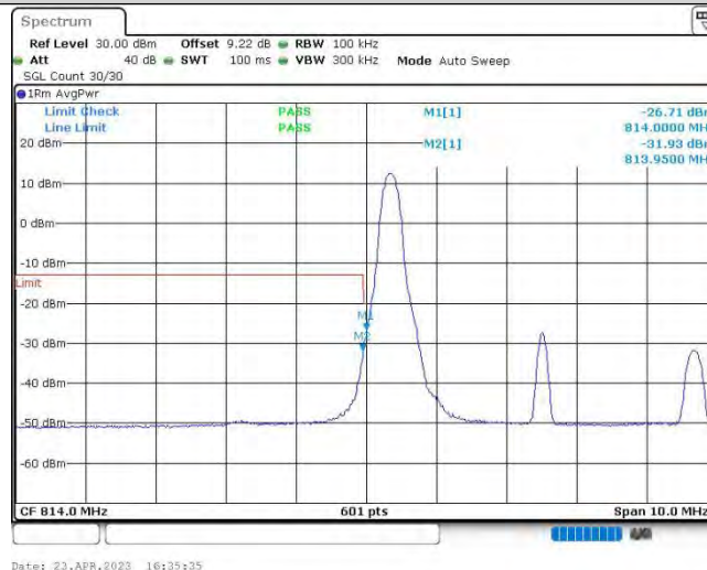
Band26@90-5MHz-16QAM-26715-1RB#0
