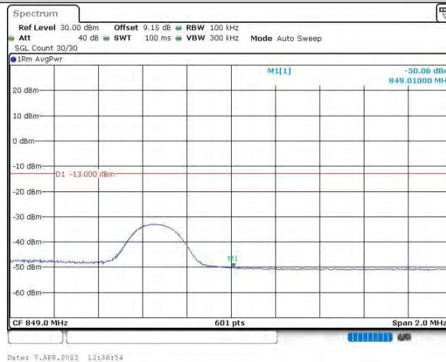
Band5-5MHz-16QAM-20625-1RB#0
