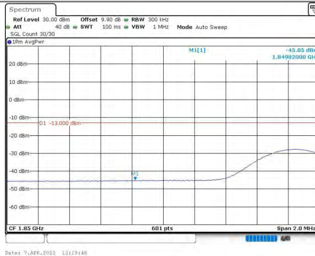
Band25-15MHz-16QAM-26115-1RB#74
