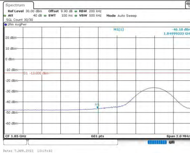
Band25-10MHz-QPSK-26090-1RB#49
