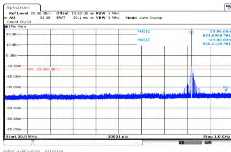
Band5-1.4MHz-QPSK-20407-1-0-Low-30-1000--34.05-PASS
