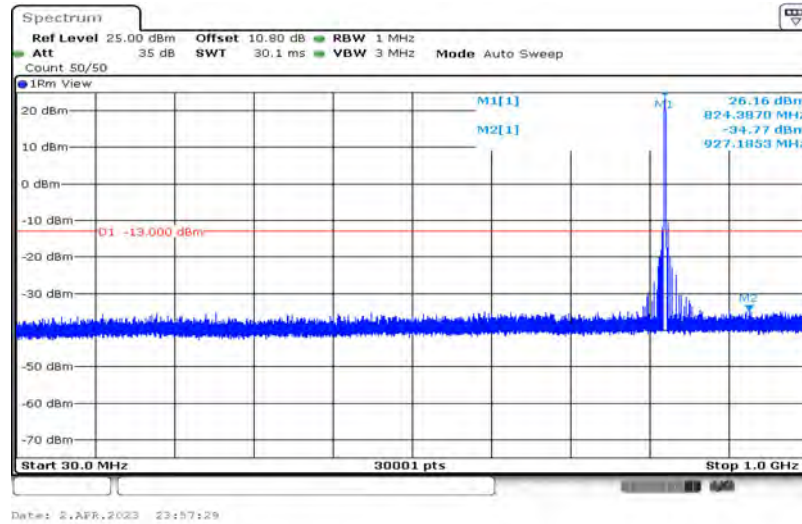
Band5-5MHz-QPSK-20425-1-0-Low-1000-5000--39.97-PASS
