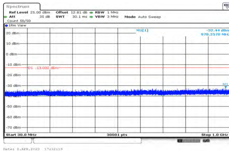
Band25-5MHz-QPSK-26665-1-0-High-30-1000--32.44-PASS
