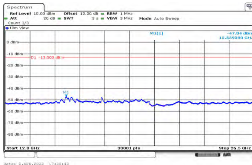
Band25-5MHz-QPSK-26365-1-0-Low-12000-26500--47.04-PASS
