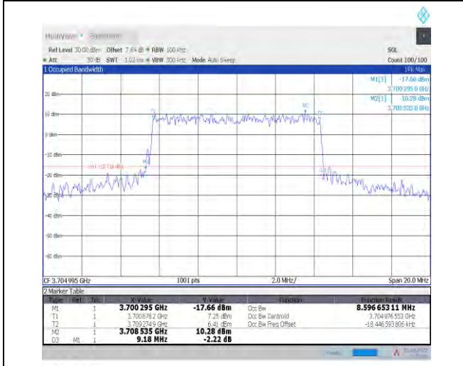
1-N77-3700-3980--30-10-L-5-DFT-256QAM-Outer_Full-24@0-Ant0-8.548-9.640-≤10-PASS
