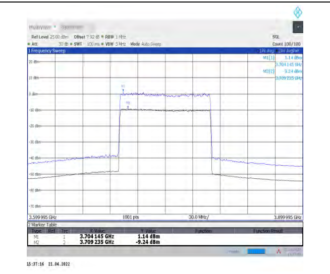
1-N77-3700-3980--30-100-L-2-CP-256QAM-Outer_Full-273@0-Ant0-10.38-100%-0.00-10.38-PASS-≤13
