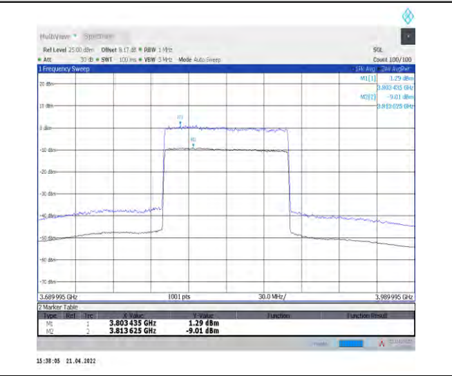
1-N77-3700-3980--30-100-M-2-CP-256QAM-Outer_Full-273@0-Ant0-10.30-100%-0.00-10.30-PASS-≤13
