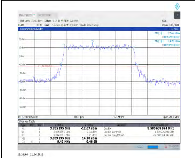
1-N77-3700-3980--30-10-M-2-DFT-PI2BPSK-Outer_Full Full-24@0-Ant0-8.581-9.420-≤10-PASS
