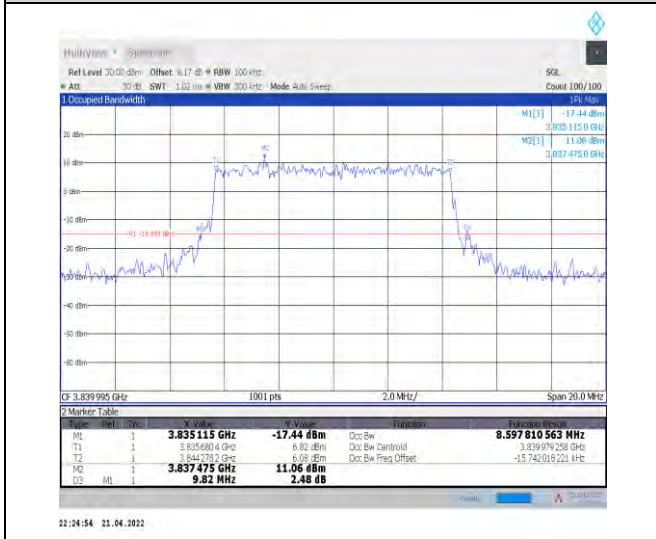
1-N77-3700-3980--30-10-M-6-CP-QPSK-Outer_Full-24@0-Ant0-8.598-9.820-≤10-PASS
