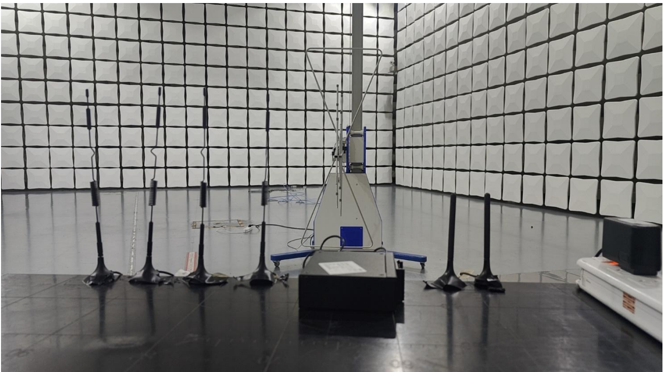
RF Radiated Test setup (30MHz~1GHz)
