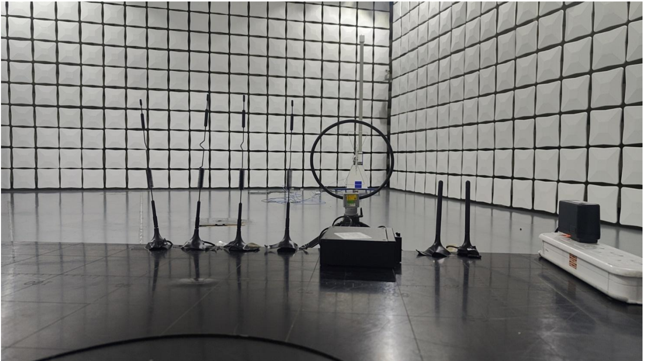
RF Radiated Test setup (9KHz~30MHz)
