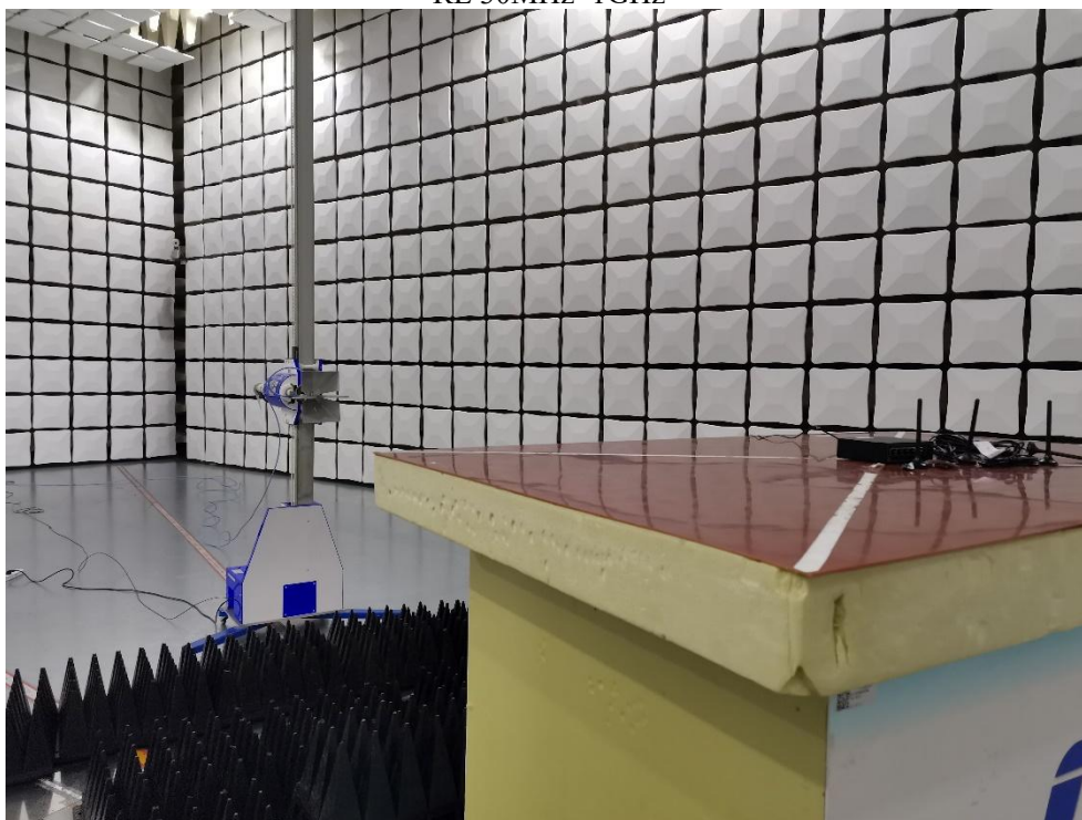
RE >1GHz
