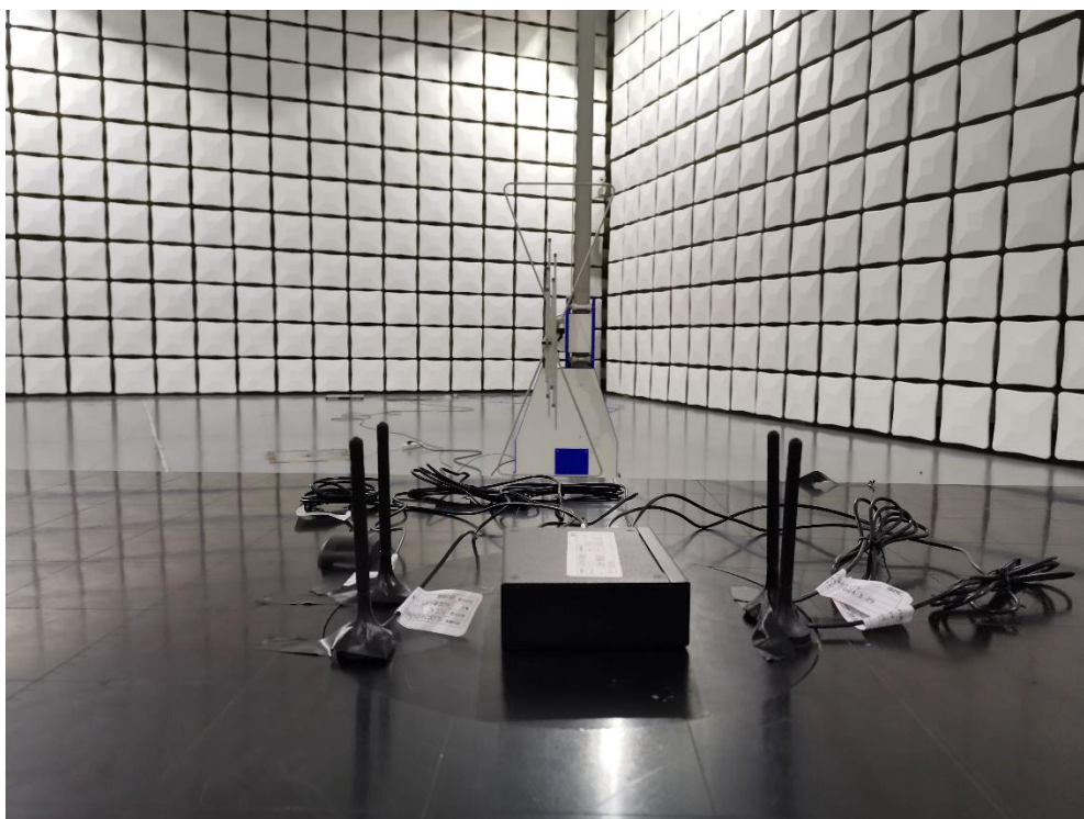
RE 30MHz~1GHz
