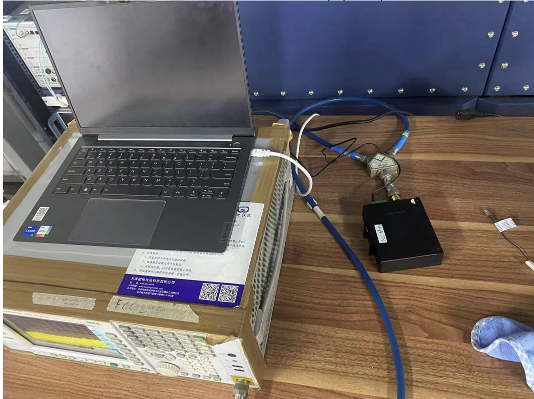
RF Conducted Test setup (LTE)
