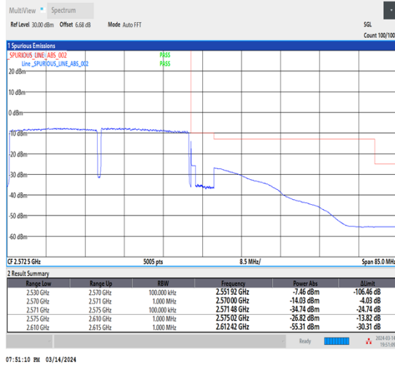
NTNV_CA_n7B_PC3_15+15_20+20_H+H_TID6_1_#1
