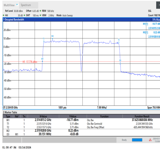
NTNV_CA_n7B_PC3_15+15_20+20_M+M_Ant1_TID5_1 _#1
