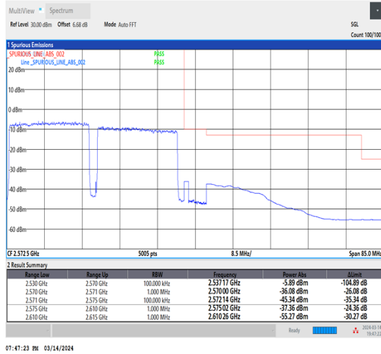
NTNV_CA_n7B_PC3_15+15_20+20_H+H_TID3_1_#1
