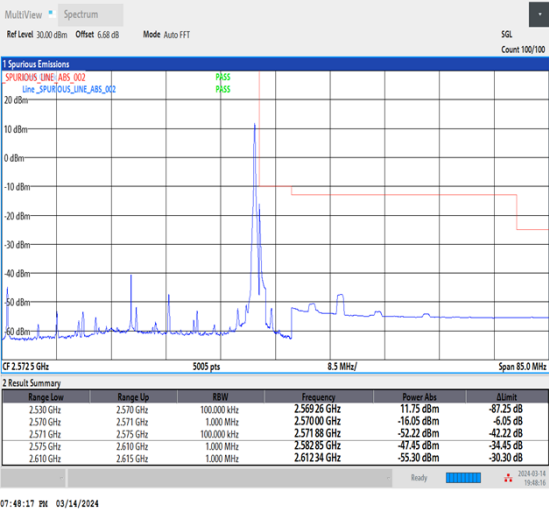
NTNV_CA_n7B_PC3_15+15_20+20_H+H_TID5_1_#1
