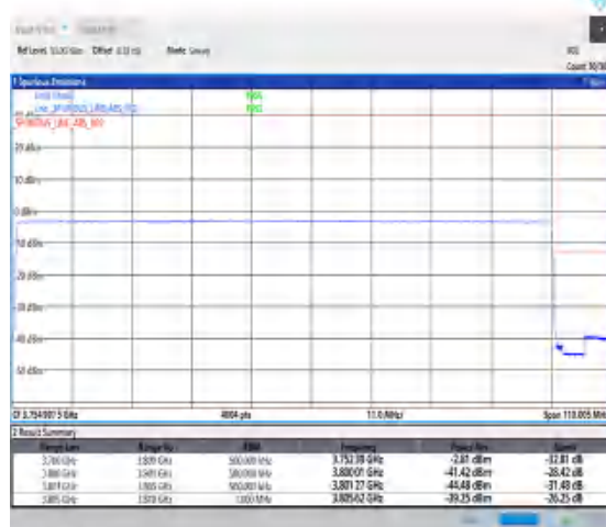
1-N78-3700-3800-30-100-H-6-CP-QPSK-Outer_Full-273@0-Ant0-1--PASS-see graph
