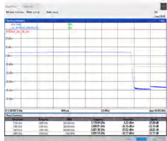
1-N78-3700-3800-30-40-H-6-CP-QPSK-Outer_Full-106@0-Ant0-1--PASS-see graph
