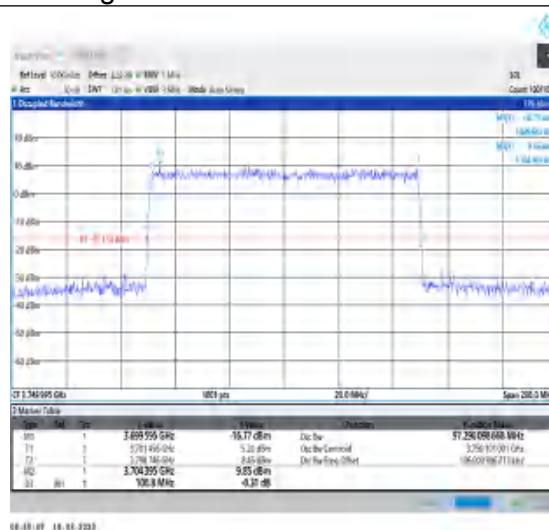
1-N78-3700-3800-30-100-L-6-CP-QPSK-Outer_Full- 273@0-Ant0-97.29-100.800-≤100-PASS
