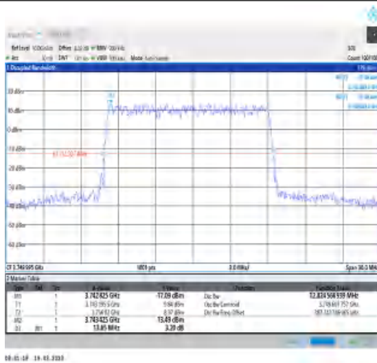
1-N78-3700-3800-30-15-M-1-DFT-QPSK-Outer_Full-36@0-Ant0-12.825-13.650-≤15-PASS
