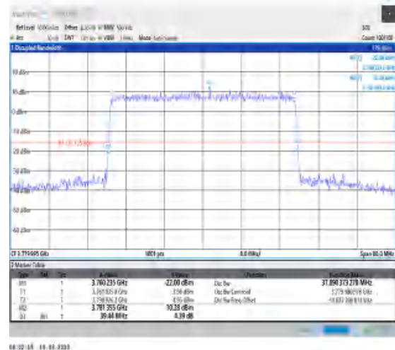
1-N78-3700-3800-30-40-H-8-CP-64QAM-Outer_Full-106@0-Ant0-37.89-39.440-≤40-PASS
