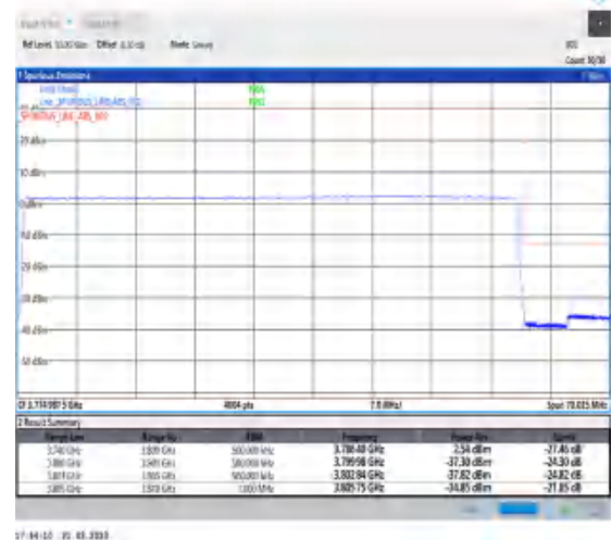
1-N78-3700-3800-30-60-H-6-CP-QPSK-Outer_Full-162@0-Ant0-1--PASS-see graph
