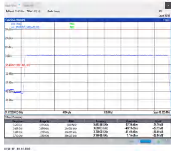
1-N78-3700-3800-30-80-L-3-DFT-PI2BPSK-Outer_Full-216@0-Ant0-1--PASS-see graph
