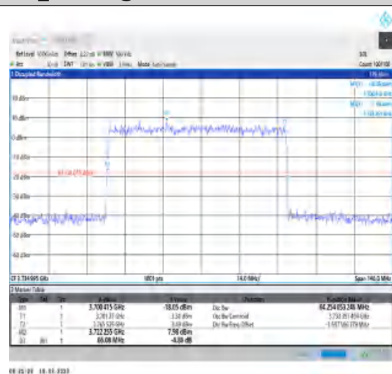
1-N78-3700-3800-30-70-L-5-DFT-256QAM-Outer_Full-180@0-Ant0-64.254-66.080-≤70-PASS
