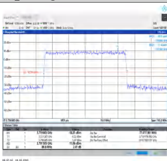
1-N78-3700-3800-30-80-H-7-CP-16QAM-Outer_Full- 217@0-Ant0-77.417-80.800-≤80-PASS
