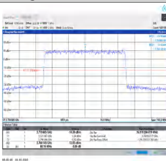
1-N78-3700-3800-30-80-H-3-DFT-16QAM-Outer_Full-216@0-Ant0-76.977-80.160-≤80-PASS
