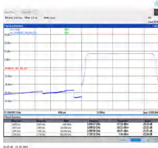
1-N78-3700-3800-30-10-L-6-CP-QPSK-Outer_Full-24@0-Ant0-1--PASS-see graph
