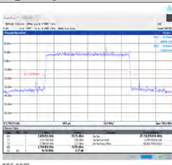
1-N78-3700-3800-30-90-L-6-CP-QPSK-Outer_Full- 245@0-Ant0-87.157-90.540-≤90-PASS
