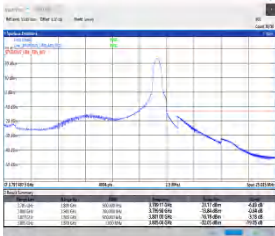
1-N78-3700-3800-30-15-H-2-DFT-PI2BPSK-Edge_1RB_Right-1@37-Ant0-1--PASS-see graph
