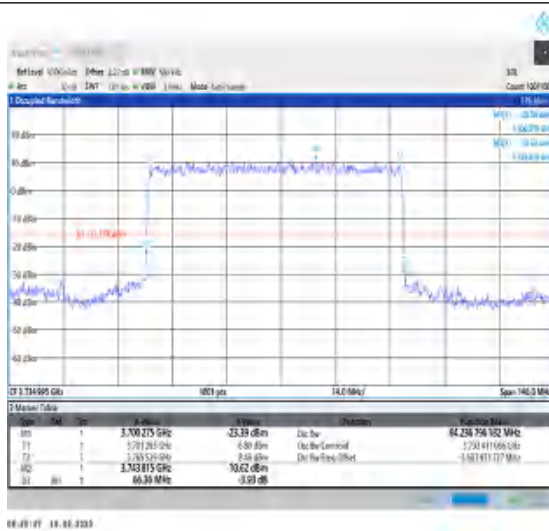
1-N78-3700-3800-30-70-L-2-DFT-PI2BPSK-Outer_Full-180@0-Ant0-64.237-66.360-≤70-PASS
