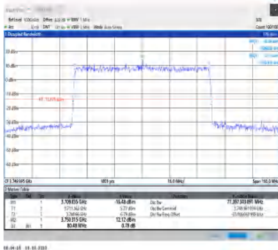
1-N78-3700-3800-30-80-M-8-CP-64QAM-Outer_Full-217@0-Ant0-77.397-80.480-≤80-PASS
