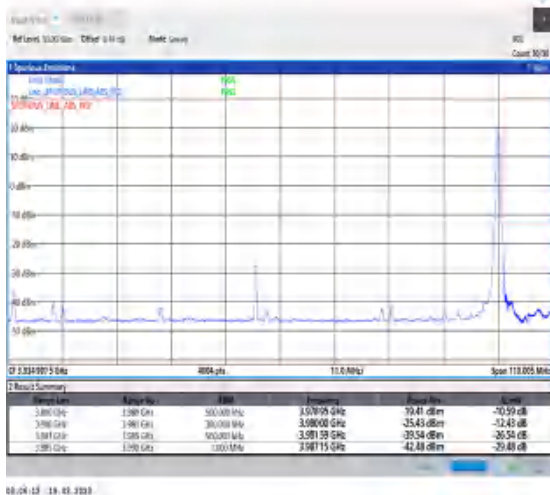
1-N77-3700-3980-30-100-H-5-CP-QPSK-Edge_1RB_Right-1@272-Ant0-1--PASS-see graph
