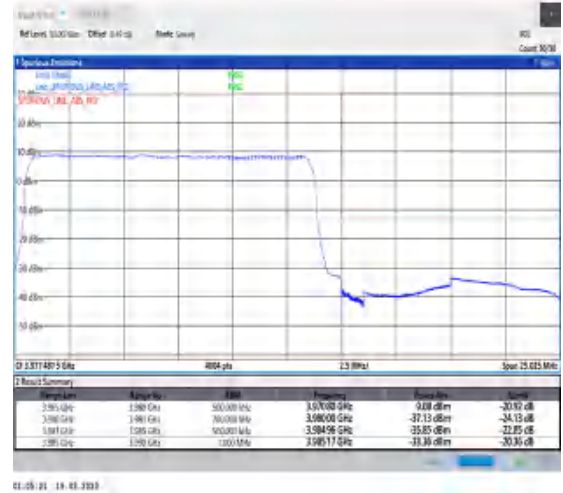
1-N77-3700-3980-30-15-H-3-DFT-PI2BPSK-Outer_Full-36@0-Ant0-1--PASS-see graph
