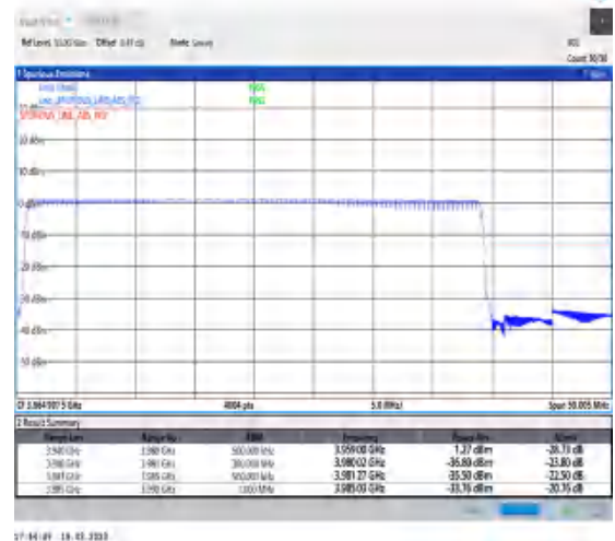
1-N77-3700-3980-30-40-H-6-CP-QPSK-Outer_Full-106@0-Ant0-1--PASS-see graph
