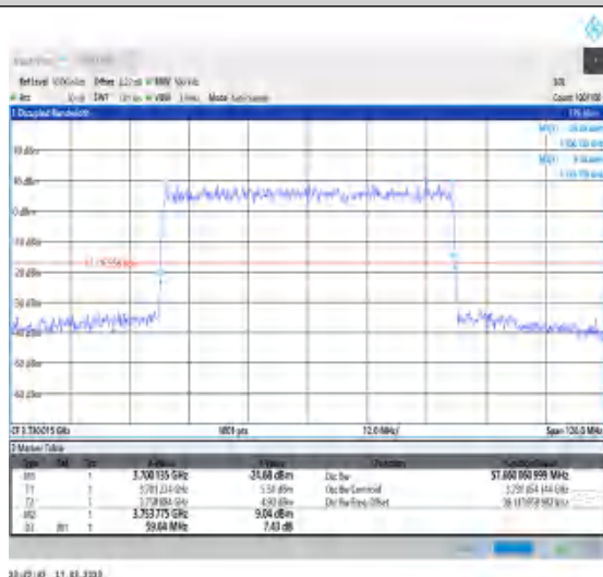
1-N77-3700-3980-30-60-L-7-CP-16QAM-Outer_Full- 162@0-Ant0-57.66-59.640-≤60-PASS
