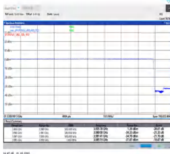
1-N77-3700-3980-30-90-H-6-CP-QPSK- Outer Full-245@0-Ant0-1--PASS-see graph
