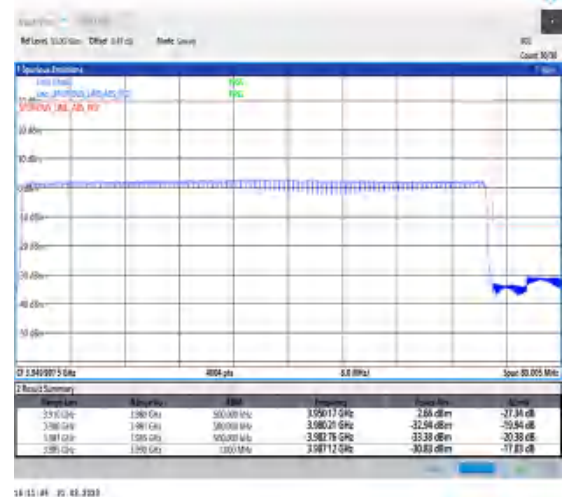
1-N77-3700-3980-30-70-H-6-CP-QPSK-Outer_Full-189@0-Ant0-1--PASS-see graph
