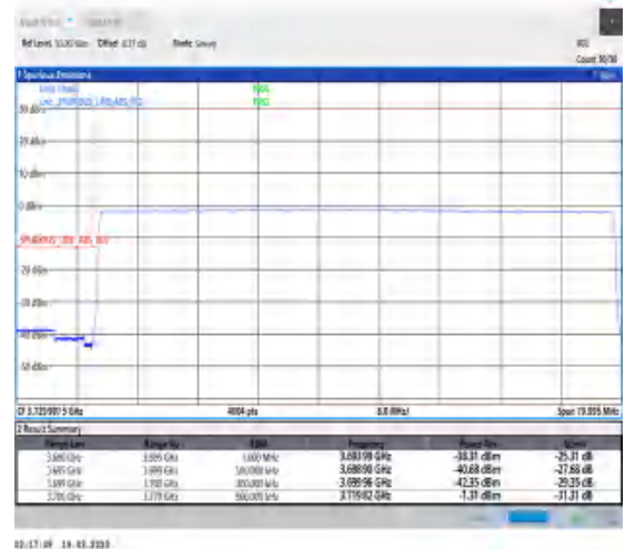
1-N77-3700-3980-30-70-L-6-CP-QPSK-Outer_Full-189@0-Ant0-1--PASS-see graph
