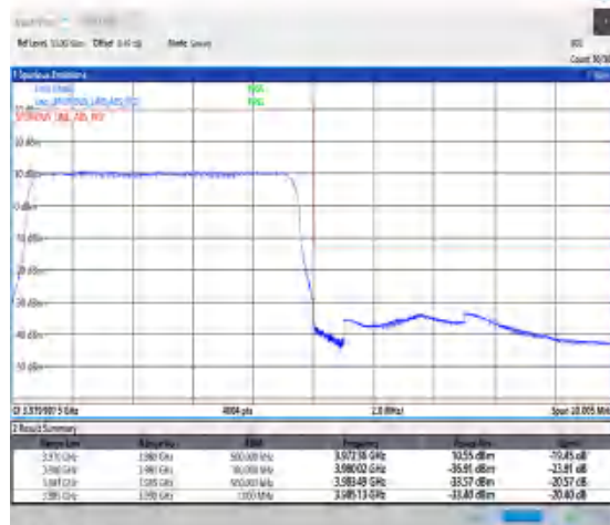
1-N77-3700-3980-30-10-H-3-DFT-PI2BPSK-Outer_Full-24@0-Ant0-1--PASS-see graph
