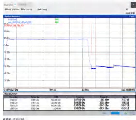
1-N77-3700-3980-30-20-H-6-CP-QPSK-Outer_Full-51@0-Ant0-1--PASS-see graph
