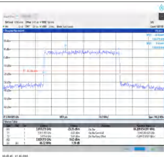
1-N77-3700-3980-30-70-H-4-DFT-64QAM- Outer Full-180@0-Ant0-64.21-66.220-≤70-PASS
